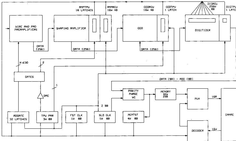
Fig. 1. Experimental Time Projection Chamber electronic block diagram showing data paths for registers and events.
