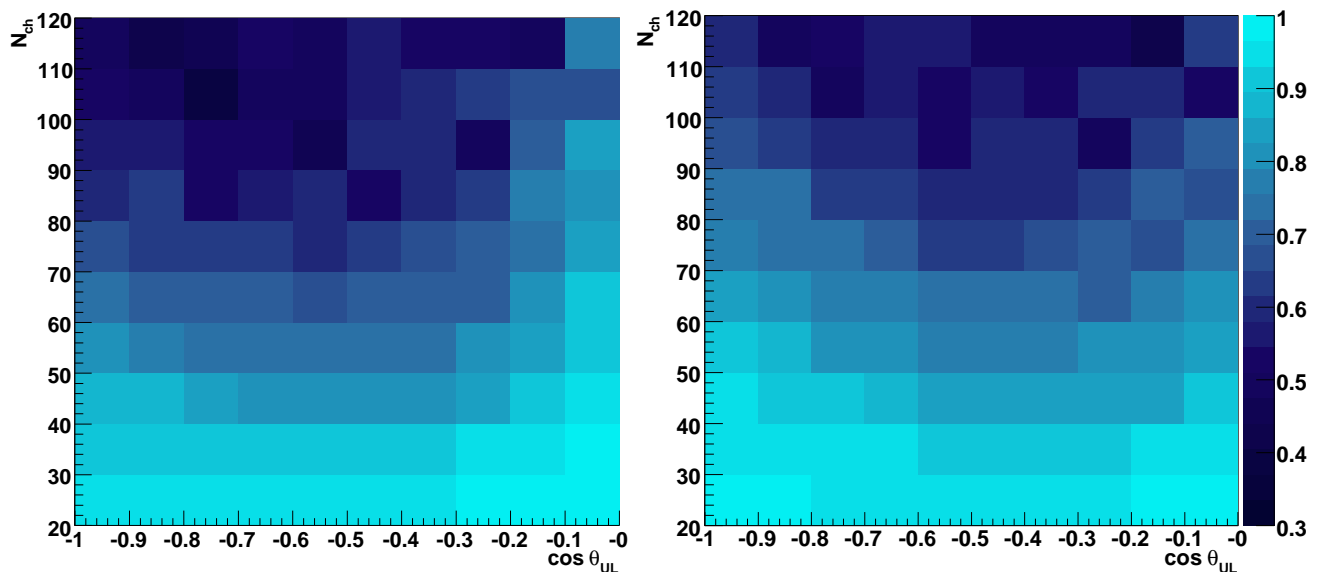
FIG. 5: Ratio of the simulated number of events given VLI (left, with n = 1 , \sin 2\xi = 1 , and \Delta\delta = 10^{-26} ) and QD (right, with n = 2 and D^* = 10^{-30} \text{ GeV}^{-1} ) to conventional oscillation predictions for the zenith angle and N_{\text{ch}} distribution.
