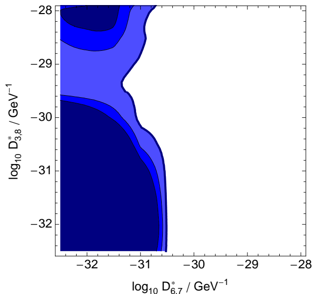
FIG. 8: 90%, 95%, and 99% CL allowed regions (from darkest to lightest) for QD effects with n = 2 .
