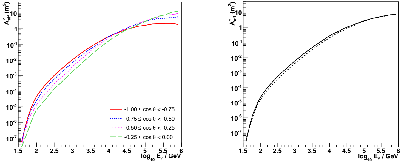
FIG. 2: Simulated detector effective area versus neutrino energy at the final analysis level. Left: \nu_{\mu} effective areas for several zenith angle ranges. Right: zenith-angle-averaged effective areas for \nu_{\mu} (solid) and \bar{\nu}_{\mu} (dotted).
