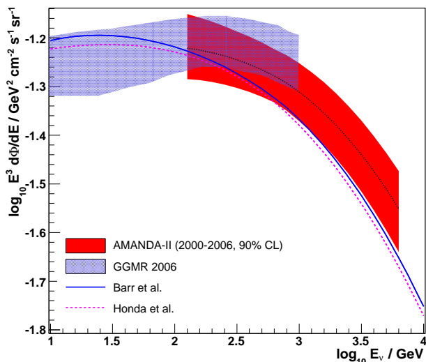
FIG. 10: Angle-averaged \nu_\mu + \bar{\nu}_\mu atmospheric neutrino flux (solid band, 90% CL from the forward-folding analysis), multiplied by E^3 to enhance features. The dotted line shows the central best-fit curve. Also shown is a previous result by González-García et al. using Super-Kamiokande data [69], as well as Barr et al. [46] and Honda et al. [13] predictions. All fluxes are shown prior to oscillations.
