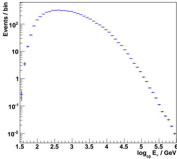
FIG. 3: Simulated \nu_{\mu} + \bar{\nu}_{\mu} energy distribution of the final event sample, assuming the Barr et al. input spectrum.
