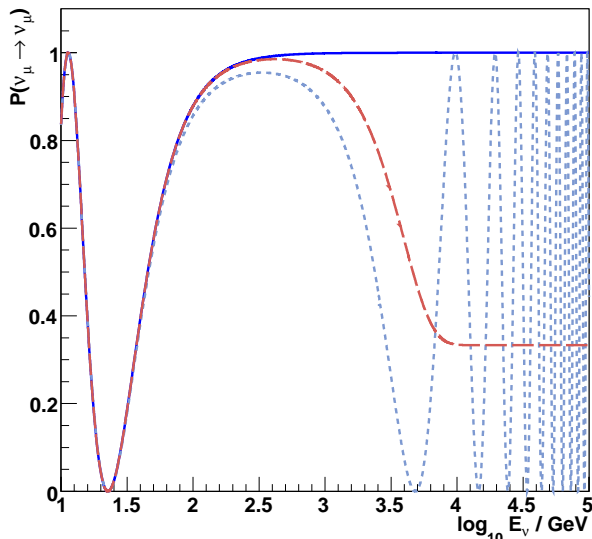
FIG. 1: \nu_\mu survival probability as a function of neutrino energy for maximal baselines ( L \approx 2R_{\text{Earth}} ) given conventional oscillations (solid line), VLI (dotted line, with n = 1 , \sin 2\xi = 1 , and \Delta\delta = 10^{-26} ), and QD effects (dashed line, with n = 2 and D^* = 10^{-30} \text{ GeV}^{-1} ).
