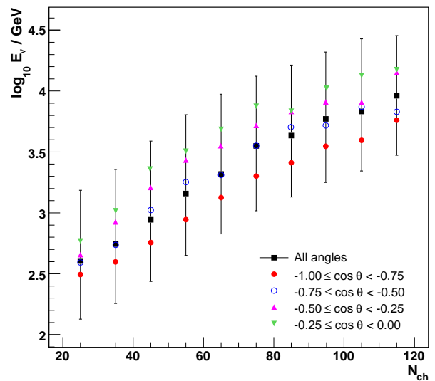
FIG. 4: Simulated profile histogram of median neutrino energy versus number of OMs hit ( N_{\text{ch}} ), both for all zenith angles below the horizon and for various zenith angle ranges. Error bars on the all-angle points represent the \pm 1\sigma spread at each N_{\text{ch}} .
