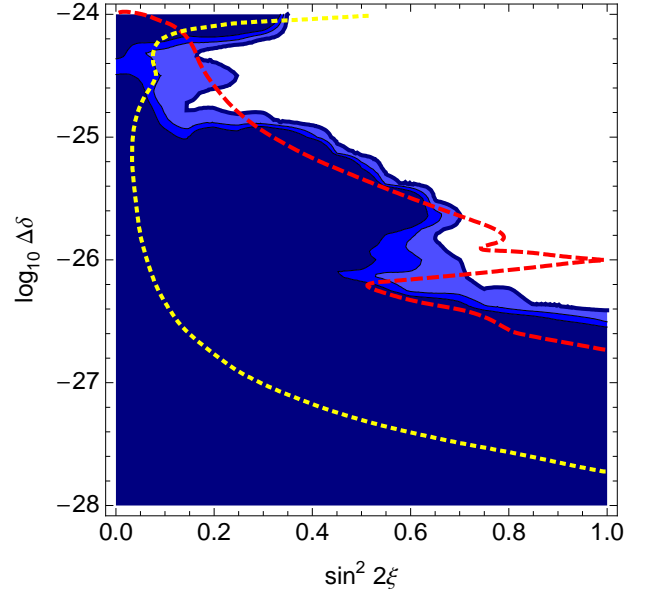
FIG. 7: 90%, 95%, and 99% CL allowed regions (from darkest to lightest) for VLI-induced oscillation effects with n = 1 . Note we plot \sin^2 2\xi to enhance the region of interest. Also shown are the Super-Kamiokande + K2K 90% contour [19] (dashed line), and the projected IceCube 10-year 90% sensitivity [68] (dotted line).
