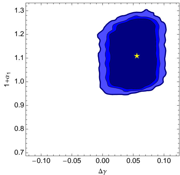
FIG. 9: 90%, 95%, and 99% allowed regions (from darkest to lightest) for the normalization (1 + \alpha_1) and change in spectral index (\Delta\gamma) of the conventional atmospheric neutrino flux, relative to Barr et al. [46]. The star marks the central best-fit point.
