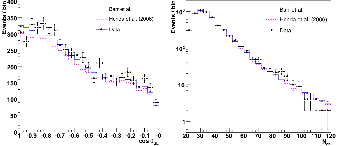
FIG. 6: Zenith angle and N_{\text{ch}} distribution of candidate atmospheric neutrino events in the final sample, compared with Barr et al. [46] and Honda et al. [13] predictions (statistical error bars).
