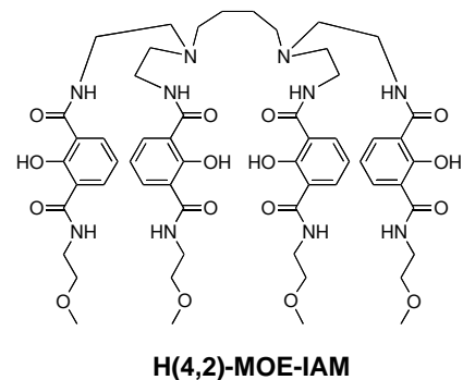
Figure 1. Chemical structure of H(2,2)-IAM (top) and monoethylene glycol (MOE)-containing analogs with varied backbones (bottom).
