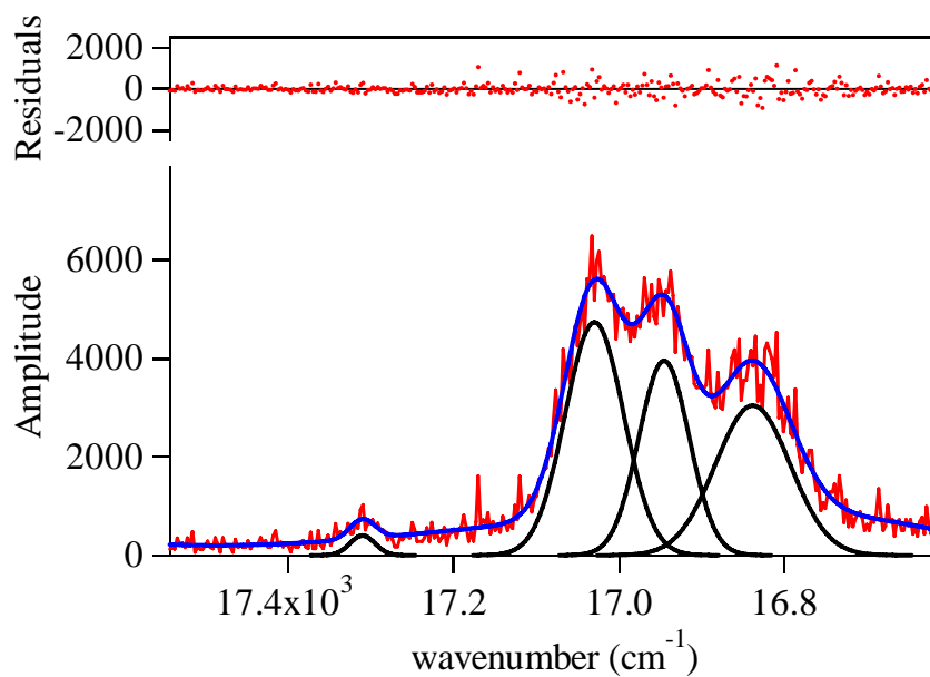
Figure 5. Expansion of the emission spectrum for the [Eu(H(2,2)-IAM-MOE)] complex in 0.1 M TRIS buffer (pH 7.4) in the J=0, 1 region and corresponding fit of the experimental spectrum to four overlapping Gaussians functions.
