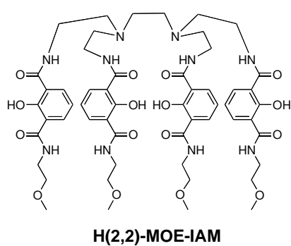
Figure 1. Chemical structure of H(2,2)-IAM (top) and monoethylene glycol (MOE)-containing analogs with varied backbones (bottom).
