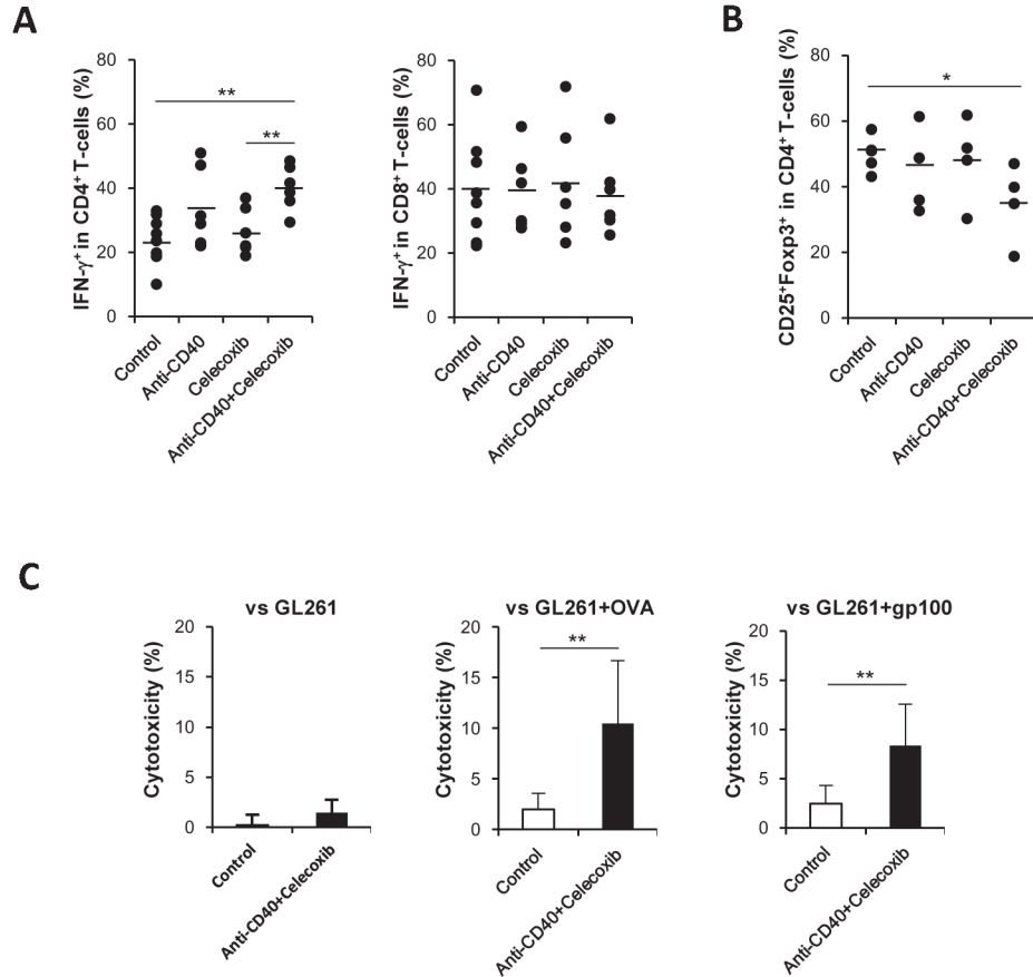
Fig. 4. The combination of anti-CD40 mAb and celecoxib improved IFN- \gamma response, reduced regulatory T-cells and induced antigen-specific cytotoxic activities
