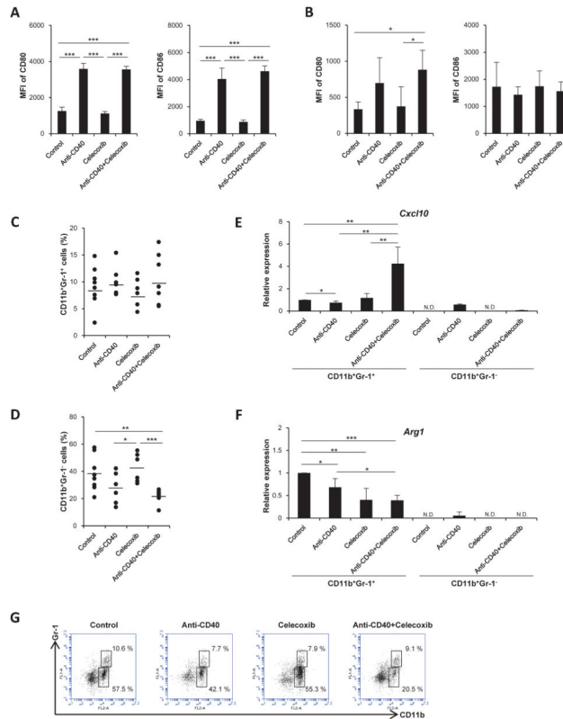
Fig. 2. The combination therapy promoted maturation and M1-like polarization of CD11b + cells C57BL/6 mice bearing Quad-GL261 glioma received the combination therapy, monotherapy with anti-CD40 mAb or celecoxib, or mock therapy on day 13 following tumor inoculation. (A) spleens and (B) BILs were harvested on day 15 from individual mice. Expression levels of CD80 and CD86 were evaluated by flow cytometry. (n=5 for Control, Anti-CD40 and Celecoxib groups; n=4 for the Anti-CD40+Celecoxib group; * P < 0.05, *** P < 0.001, t -test). (C and D) Frequencies of CD11b + Gr-1 + and CD11b + Gr-1 - cells in the brain were evaluated by flow cytometry on day 5 after therapy. (n=8 for Control, n=6 for monotherapy with Anti-CD40 or Celecoxib, in each group; n=7 for Anti-CD40+Celecoxib; * P < 0.05, ** P < 0.01, *** P < 0.001, t -test). (E and F) BILs were harvested on day 5 post-treatment. CD11b + Gr-1 + and CD11b + Gr-1 - BILs were purified from pooled BILs (n=3–4 in each group) by cell sorting and mRNA expression levels for Cxcl10 and Arg1 were determined by real-time PCR. Bars and error bars indicate the mean and SD, respectively, from two independent experiments. (N.D., not detected; * P < 0.05, ** P < 0.01, *** P < 0.001, t -test) (G) Representative flow data of BILs on CD11b + Gr-1 + and CD11b + Gr-1 - cells on day 5 post-treatment.
