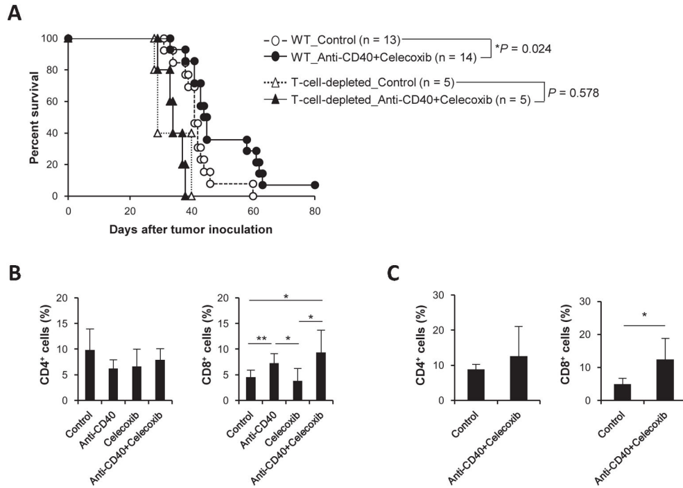
Fig. 3. T-cells were responsible in the observed anti-glioma activity of the combination regimen (A) Wild-type (WT) or CD8-deficient mice depleted of CD4 + cells (T-cell-depleted) received intracranial inoculation of Quad-GL261 glioma cells, and then received anti-CD40 mAb i.p. on days 13 and 23, and celecoxib via diet through days 13–33. Kaplan-Meier plot illustrates the survival. (* P < 0.05, Log-rank test) (B) C57BL/6 mice bearing Quad-GL261 cells, or (C) de novo Sleeping Beauty gliomas received anti-CD40 mAb and/or celecoxib. BILs were harvested on day 5 after treatment and analyzed by flow cytometry. Bars and error bars indicate the mean and SD, respectively, from three independent experiments. [(B) n=8 for Control, n=6 for each of Anti-CD40 and Celecoxib groups, n=7 for Anti-CD40+Celecoxib, (C) n=5 and 6 for Control and Anti-CD40+Celecoxib, respectively; * P < 0.05, ** P < 0.01, t -test]
