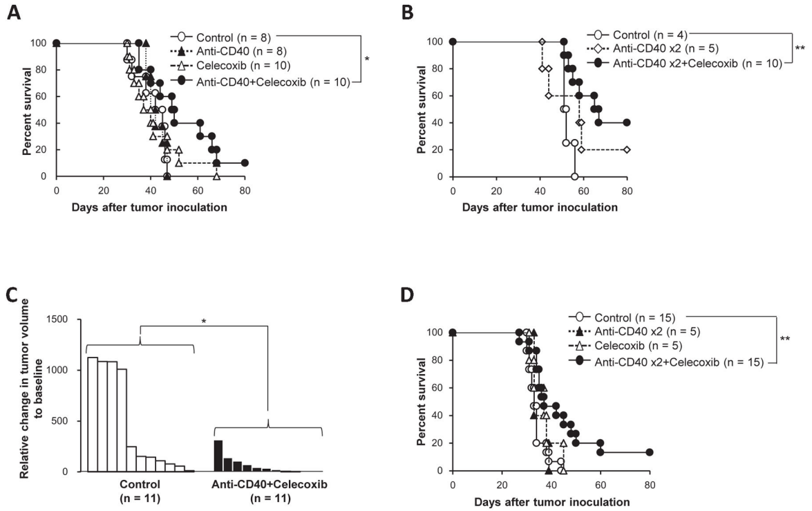
Fig. 1. Agonistic anti-CD40 mAb in combination with celecoxib significantly prolonged survival C57BL/6 mice bearing Quad-GL261 glioma received anti-CD40 mAb i.p. on (A) day 13 or (B) days 13 and 23, and/or celecoxib via diet through days 13-33. Kaplan-Meier plot illustrates the survival. (* P < 0.05 , ** P < 0.01 , Log-rank test) (C) C57BL/6 mice bearing established de novo gliomas received the combination therapy or mock treatment. Relative change in tumor volume from day -T1 (baseline; on the day before the treatment started) to day T15 is shown for each mouse as a waterfall plot. (n = 11 in each group; * P < 0.05 , t -test) (D) C57BL/6 mice bearing SB28 glioma received anti-CD40 mAb i.p. on days 13 and 23 and/or celecoxib via diet through day 13 through day 33. Kaplan-Meier plot illustrates the survival. (** P < 0.01 , Log-rank test)
