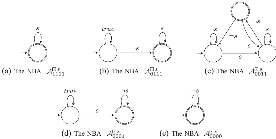
Fig. 1 The Büchi automata \mathcal{A}_\beta^{\Box s} constructed in Step 1 of our monitor construction
