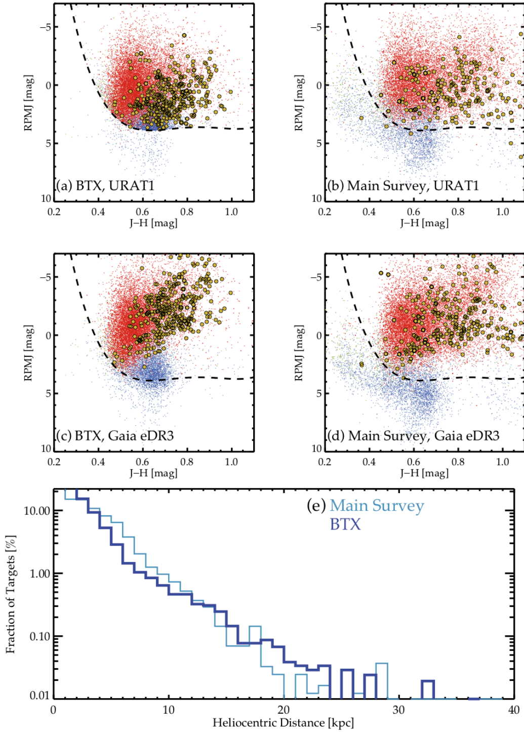
Figure 7. RPMJ selection criteria applied in the outer disk (left column) and the same visualized for the main survey sample in the same region of the sky (right column) for different proper motion catalogs, at top URAT1 and middle Gaia eDR3 (Gaia Collaboration et al. 2020). The dashed line shows the RPMJ division given in Equation 2. The points are color-coded by spectroscopic giants (red), spectroscopic sub-giants (green), and spectroscopic dwarfs (blue) with the larger symbols indicating spectroscopic giants at heliocentric distances greater than 12 kpc. The BTX and Main Survey samples both have \sim 18,000 stars. The BTX sample has systematically bluer colors than the main survey, though the main survey sample does have higher-extinction sight-lines. (e) Fraction of targets at a given heliocentric distance for the main survey (thin blue) and the BTX (thick purple).
