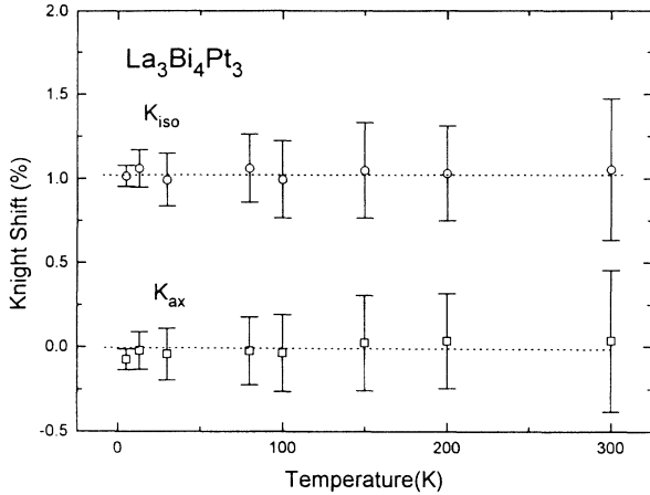
FIG. 7. Temperature dependence of the isotropic and axial Knight shifts in \text{La}_3\text{Bi}_4\text{Pt}_3 .
