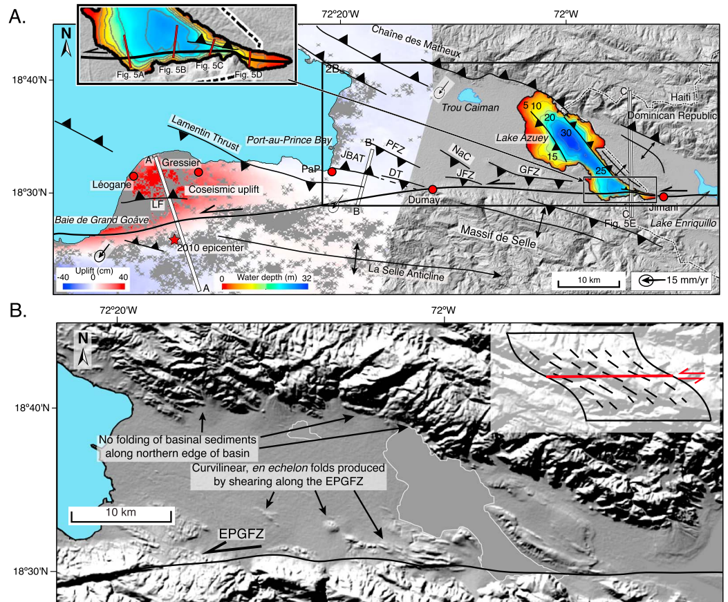
Figure 2. Structure of the EPGFZ in eastern Haiti. (a) Faults and folds along a 15-km-wide corridor parallel to the EPGFZ superimposed on a modified DEM and Interferometric Synthetic Aperture Radar (InSAR) surface deformation map (courtesy of Eric Fielding at JPL; Hayes et al., 2010). Chirp bathymetry of the Lake Azuey is also shown. GPS vectors are from Calais et al. (2010). PFZ = Port-au-Prince fault zone; DT = Dumay thrust; JBAT=John Brown Avenue thrust; NaC = Nan Cadastre thrust; JFZ = Jacquet fault zone; GFZ = Ganthier fault zone; LF = Léogâne fault; EPGFZ = Enriquillo-Plantain Garden fault zone; DEM = digital elevation model. Line A–A': Cross section along the blind Léogâne thrust fault (shown in Figure 3); Line B–B': Cross section of north Port-au-Prince urban area (shown in Figure 3). (b) Shaded DEM of the northern deformed belt in the Cul-de-Sac showing en echelon and curvilinear folds striking west-northwest obliquely with respect to the EPGFZ and plunging beneath undeformed sediments occupying the center of the Cul-de-Sac Valley. The inset schematic diagram of shearing along a left-lateral strike-slip fault is from Odonne and Vialon (1983).
