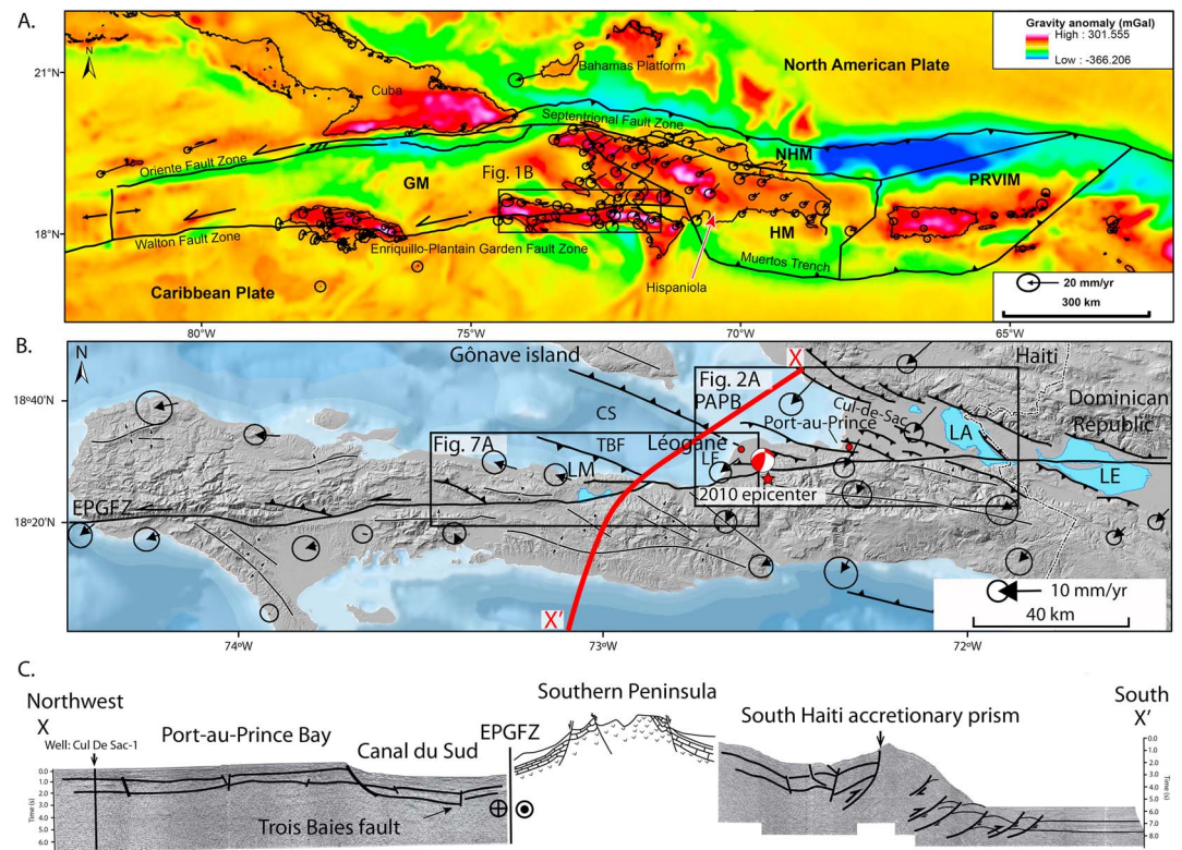
Figure 1. Tectonic setting of the northeastern Caribbean and Enriquillo-Plantain Garden fault zone (EPGFZ) in southern Haiti. (a) Free-air gravity anomaly map of the Greater Antilles (Cuba, Jamaica, Hispaniola, and Puerto Rico) in the northeastern Caribbean ( http://topex.ucsd.edu ) with gravity lows marking zones of subduction or thrusting along major faults (black lines) of the North America-Caribbean plate boundary. Arrows with error ellipses from Calais et al. (2016) are GPS vectors showing the direction and velocity of the large North American plate, the Bahamas platform, and intervening microplates relative to a fixed Caribbean plate. Microplates with variable relative motions occupy the 200-km-wide, transpressional, plate boundary zone and include the following: NHM = North Hispaniola microplate; HM = Hispaniola microplate; GM = Gonâve microplate; PRVIM = Puerto Rico-Virgin Islands microplate. Box shows more detailed map of the EPGFZ shown in (b). (b) Regional structure map of the southern peninsula of Haiti with the active, left-lateral Enriquillo-Plantain Garden fault zone (EPGFZ) from the Lake Enriquillo in the east to the western tip of the southern peninsula. The centroid moment tensor (CMT) mechanism is from Douilly et al. (2013). From east to west, key lakes and marine embayments aligned parallel and overlying the EPGFZ include the following: LE = Lake Enriquillo, Dominican Republic; LA = Lake Azuey, Haiti; PAPB = Port-au-Prince Bay; CS = Canal du Sud; TBF = Trois Baies fault; LM = Lake Miragoâne; LF = Léogâne fault. Boxes show more detailed maps of the structure of the EPGFZ and its secondary faults shown in Figures 2a and 7a. (c) Composite, multichannel seismic reflection line (acquired by Canadian Superior Energy Inc.) located as the red line X-X' in (b) that shows an unfolded area of high-angle faults in the Canal du Sud tied to the offshore Cul-de-Sac-1 well, the Trois Baies fault, the EPGFZ, the anticlinal structure of the southern peninsula, and a large, south verging accretionary prism along the south coast of the southern peninsula. The depth scale for this section is in two-way, travel time.
