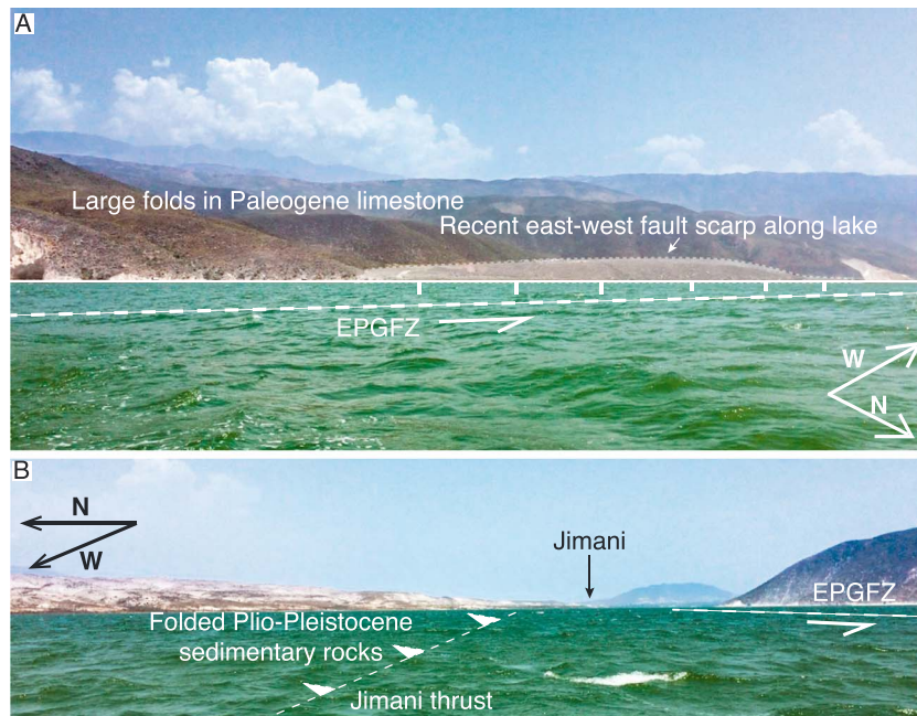
Figure 4. Geologic setting of Lake Azuey, Haiti. (a) To the south, the green-colored, brackish waters of Lake Azuey are bound by the EPGFZ which forms a sharp boundary with 2-km-high folded limestone of Paleogene age that forms the smooth surfaces on the skyline. A fault strand of the EPGFZ marks the south edge of Lake Azuey, while other parallel strands of the EPGFZ underlie the southern part of the lake as schematically shown. (b) To the north of the lake folded, Plio-Pleistocene strata form the uplifted, 0- to 30-m-high isthmus that separates Lake Azuey (15-m ASL) from Lake Enriquillo (46-m BSL) located 1 km to the east. Approximate locations of the EPGFZ and the Jimani thrust fault are shown. EPGFZ = Enriquillo-Plantain Garden fault zone.
