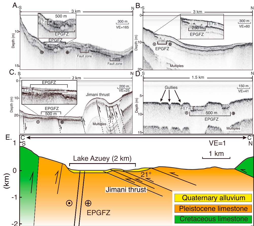
Figure 5. Chirp sonar profiles showing the trace of the EPGFZ in the southern part of Lake Azuey and its relationship with a newly described thrust we have named the Jimani thrust. (a–d) Cross sections indicated in the inset of Figure 2a. The EPGFZ beneath Lake Azuey forms a 250- to 500-m-wide zone that can be traced as a lineament to the east and west of Lake Azuey (Figure 2). The green and red horizons represent two distinguish stratigraphic layers. The two strands of the EPGFZ are buried by 0.7 m of Holocene sediment and are extrapolated to be 270 years old since their last rupture when an average sedimentation rate of 2.6 mm/year based on cores from Lake Enriquillo is assumed. Folds associated with the Jimani thrust are interpreted as fault propagation folds above northeast dipping thrust faults. (e) Cross section based on both sonar survey and the surface mapping (Mann et al., 1991) showing north and south dipping, reverse faults deforming Plio-Pleistocene sedimentary rocks. EPGFZ = Enriquillo-Plantain Garden fault zone.
