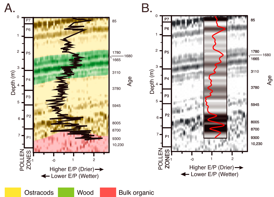
Figure 9. Core data from Lake Miragoâne. (a) Tie between chirp sonar and core with radiocarbon age control back to 10,230 years BP (Higuera-Gundy et al., 1999). Cyclicity is related to changes in lithology related to alternating wet and dry periods as shown. Yellow areas are shallow marine to freshwater, and green areas contain wood debris and may mark a period when the lake was dry. (b) Low-pass filtered E/P log (red) and the synthetic sonar profile generated from the low-pass filtered E/P log used as an acoustic impedance. The chirp sonar profiles are from the location of the red bar in the Figures 8b and 8c.
