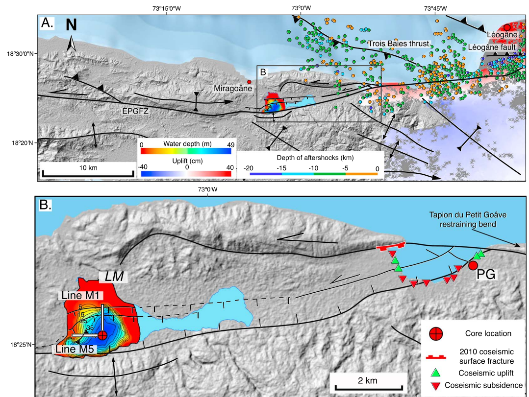
Figure 7. Structure and 2010 coseismic surface deformation of the western segments of the EPGFZ. (a) Fault map (Cowgill et al., 2012; Prentice et al., 2010) and map of 2010 aftershocks (Douilly et al., 2013) in Miragoâne-Léogâne region overlain with an InSAR image (courtesy of Eric Fielding at JPL; Hayes et al., 2010). (b) Zoom of the area of Petit Goave and Lake Miragoâne showing the structure and bathymetry of the 14 km 2 , pull-apart basin underlying Lake Miragoâne during this study and details of the 2010 surface fracturing and coseismic subsidence in the Petit Goave Bay (Hornbach et al., 2010; Prentice et al., 2010). LM = Lake Miragoâne; PG = Petit Goave; EPGFZ = Enriquillo-Plantain Garden fault zone.
