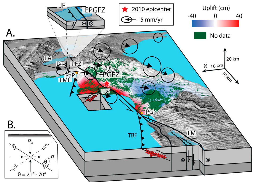
Figure 10. Schematic diagram of the conjugate thrust-fault model for the 10- to 15-km-wide belt of transpressional deformation along the northern edge of the EPGFZ. (a) Three-dimensional block diagram showing the structural aftershocks and the late Holocene strain partitioning in a 40-km-wide zone along a 120-km-long segment of the EPGFZ. Black arrows show the southwest direction of the GPS vectors relative to the Caribbean plate (Calais et al., 2016). The 2010 InSAR-derived surface deformation map (provided by Eric Fielding at JPL; Hayes et al., 2010) shows a large component of shortening accommodated on a 40-km-wide zone of oblique thrusts and folds north of the EPGFZ. Aftershock pattern shown in the cross section shows the northeastward dip of the en echelon. Léogâne thrust adjacent to the EPGFZ uplifted the topographically lower basinal area to the north of the EPGFZ and depressed the mountainous area to the south of the EPGFZ. The alternating dip of the en echelon thrusts is related to their origin as conjugate thrust faults in a highly transpressional setting. PaP = Port-au-Prince; PG = Petit Goave; LA = Lake Azuey; LM = Lake Miragoâne-Léogâne; JF = Jimani thrust fault; DT = Dumay thrust; PFZ = Port-au-Prince fault zone; LMF = Lamartin thrust fault; TBF = Trois Baies thrust fault; LF = Léogâne fault; EPGFZ = Enriquillo-Plantain Garden fault zone. (b) Schematic diagram, modified from Sibson (2012), of the conjugate thrust faults.
