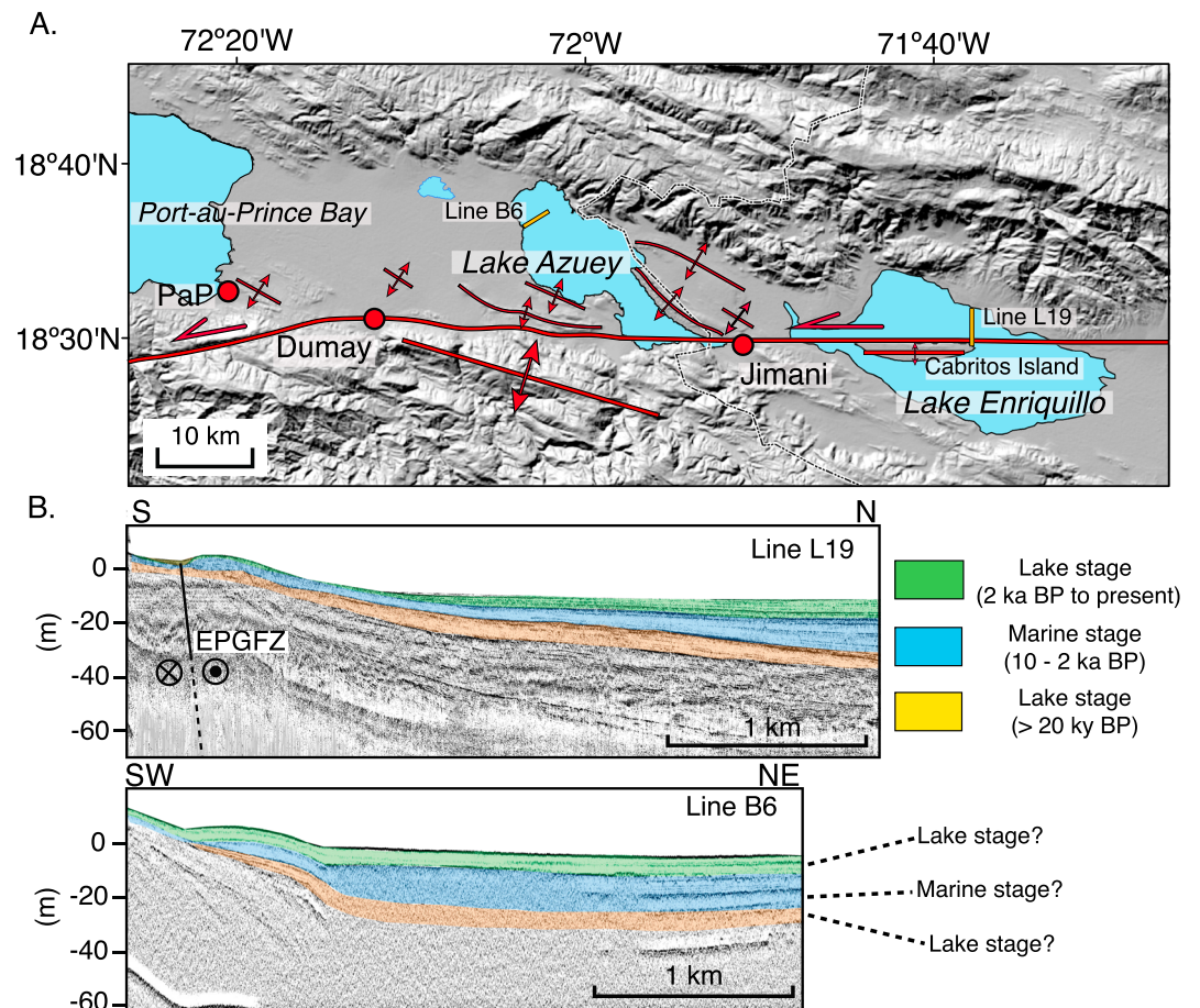
Figure 6. Structure of the EPGFZ in eastern Haiti and westernmost Dominican Republic. (a) Structural map of Lakes Azuey (surface 15-m ASL) and Lake Enriquillo (surface 46-m BSL) are presently separated by a shallow sill 30-m ASL in the isthmus near the town of Jimani. (b) Comparison of two Chirp lines from Lake Enriquillo by Rios et al. (2013) 3-km-long Line L19) and from our study of Lake Azuey (4-km-long Line B6). Chirp profiles from both lakes show three, major, stratigraphic sequences. Ages of units are known from Lake Enriquillo through both exposures around the subsea level lake and from lake coring by Rios et al. (2013). EPGFZ = Enriquillo-Plantain Garden fault zone.
