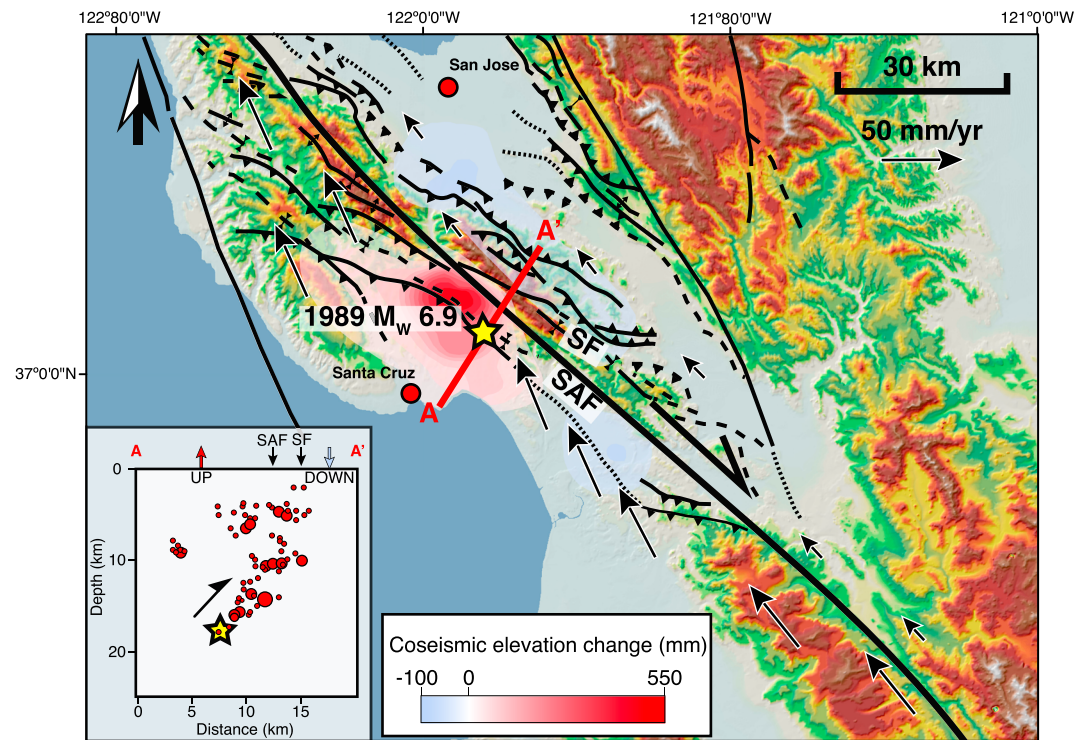
Figure 11. Structural map of the southern San Francisco Bay region, the coseismic elevation, and the aftershock cross section of 1989 M_w 6.9 Loma Prieta earthquake. The selected GPS vectors relative to a fixed North America plate are from University Navstar Consortium (2009). The coseismic elevation change and aftershock cross section are modified from Marshall et al. (1991). SAF = San Andreas Fault; SF = Sargent Fault. Aftershock pattern in the cross section shows that the southwest dip of the en echelon thrust adjacent to the San Andreas fault uplifted the topographically lower basinal area and depressed the mountainous area to the northeast of the San Andreas fault.
