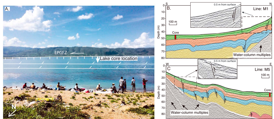
Figure 8. Geologic setting and sonar profiles from Lake Miragoâne. (a) View looking south across the 12-km-wide and 42.8-m-deep, freshwater lake. The 2-km-high ridge along the southern edge of the lake is the cumulative topographic scarp associated with the southernmost strand of the EPGFZ. The 7-m-long core was taken by Higuera-Gundy et al. (1999) but was not collected from the deepest part of the lake. (b) North-south trending line M1 (location shown in Figure 7b). (c) East-west trending line M5 (location shown in Figure 7b). In the lines shown in (b) and (c), the strands of the EPGFZ are both buried by 0.5 m of sediment. EPGFZ = Enriquillo-Plantain Garden fault zone.
