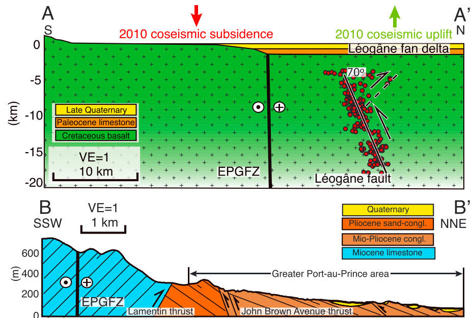
Figure 3. Style of late Neogene, transpressional deformation in the northern belt along two transects shown in Figure 2. (A–A′) Aftershocks of the 2010 earthquake (Douilly et al., 2015, 2013) along the blind Léogâne thrust fault reveal conjugate reverse faults with the dominant slip occurring on the north dipping fault. Coseismic uplift during the 2010 earthquake elevated the northern basinal area and depressed the mountains south of the EPGFZ. (B–B′) Cross section based on surface mapping (Bachhuber et al., 2010; Butterlin, 1960; Cox et al., 2011; McHugh et al., 2011; Rathje et al., 2011, 2014; Saint Fleur et al., 2015) showing both north and south dipping reverse faults deforming Plio-Pleistocene sedimentary rocks that underlie the Greater Port-au-Prince area. EPGFZ = Enriquillo-Plantain Garden fault zone.
