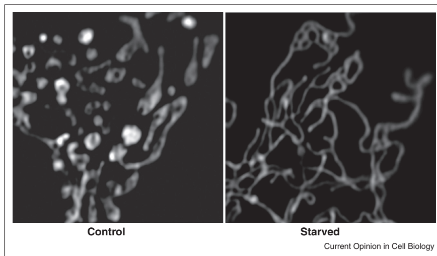
Starvation leads to unopposed mitochondrial fusion. Mouse embryo fibroblasts transfected with mitoRFP were incubated in full nutrient medium (Control), or starvation medium (Starved) for six hours. Starved cells show a continuous network of mitochondria. Cells were fixed and images acquired by Structured Illumination Microscopy. Images courtesy of Angelika Rambold and Jennifer Lippencott-Schwartz.
