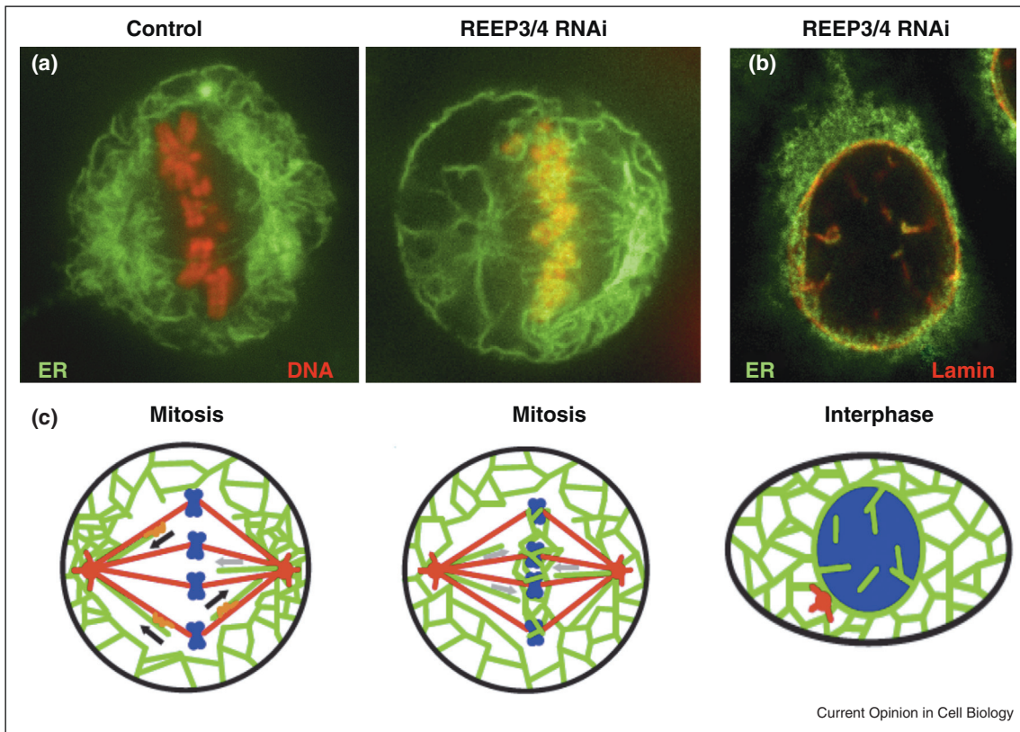
Depletion of REEP3/4 causes accumulation of ER on mitotic chromosomes and leads to intranuclear membranes and lamina. (a) HeLa cells expressing RFP-histone (red) to label the DNA and GFP-Sec61 (green) to mark the ER were subjected to control or REEP3/4 RNAi and imaged during mitosis. Note the colocalization of ER and mitotic chromosomes in the absence of REEP3/4. (b) An interphase REEP3/4 RNAi-treated HeLa cell expressing GFP-Sec61 (green) was fixed and stained for nuclear lamin B1 (red). Both NE markers are aberrantly localized to structures inside the nucleus. (c) Schematic of phenotypes with microtubules in red, DNA in blue and ER in green. Adapted from Ref. [33**]. Images courtesy of Anne-Lore Schlaitz and Rebecca Heald.
