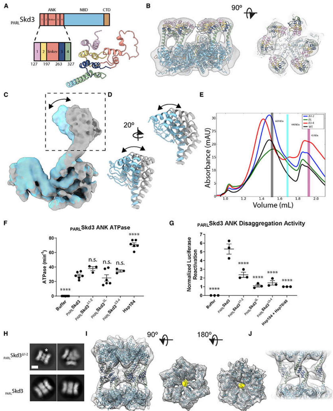
Figure 3. The ANK mediates head-to-head contacts required for dodecamerization (A) Schematic and model of PARL_Skd3 ANK, colored-based repeat number and linker. (B) Side (left) and top (right) views of the filtered class 1 map and docked model, colored as in (A), identifying ANK position. (C and D) Overlay of two different classes resolved from focus classification around P3 identifying rotation of the ANK region (arrow). (E) SEC of PARL_Skd3 (black), PARL_Skd3 1-2 (blue), PARL_Skd3 L (green), and PARL_Skd3 3-4 (red) incubated with ATPγS and casein. Vertical bars indicate molecular weight standards: (F) ATPase activity for PARL_Skd3 ANK ATPase. **** p < 0.0001, n.s. = not significant. (G) Normalized Luciferase Reactivation for PARL_Skd3 ANK Disaggregation Activity. **** p < 0.0001. (H) Microscopy images of PARL_Skd3 Δ1-2 (top) and PARL_Skd3 (bottom) showing dodecamer formation. An asterisk (*) is present in the top-left image. (I and J) 3D models of the dodecamer with ANK regions highlighted in yellow. Rotation arrows for 90° and 180° are shown.
