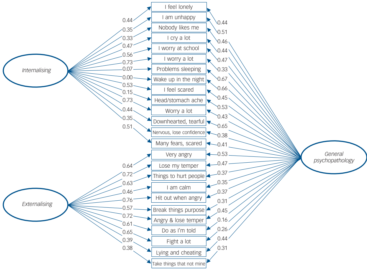
Fig. 1 Bi-factor model with the item loadings onto the internalising and externalising dimensions and the general psychopathology bi-factor.
