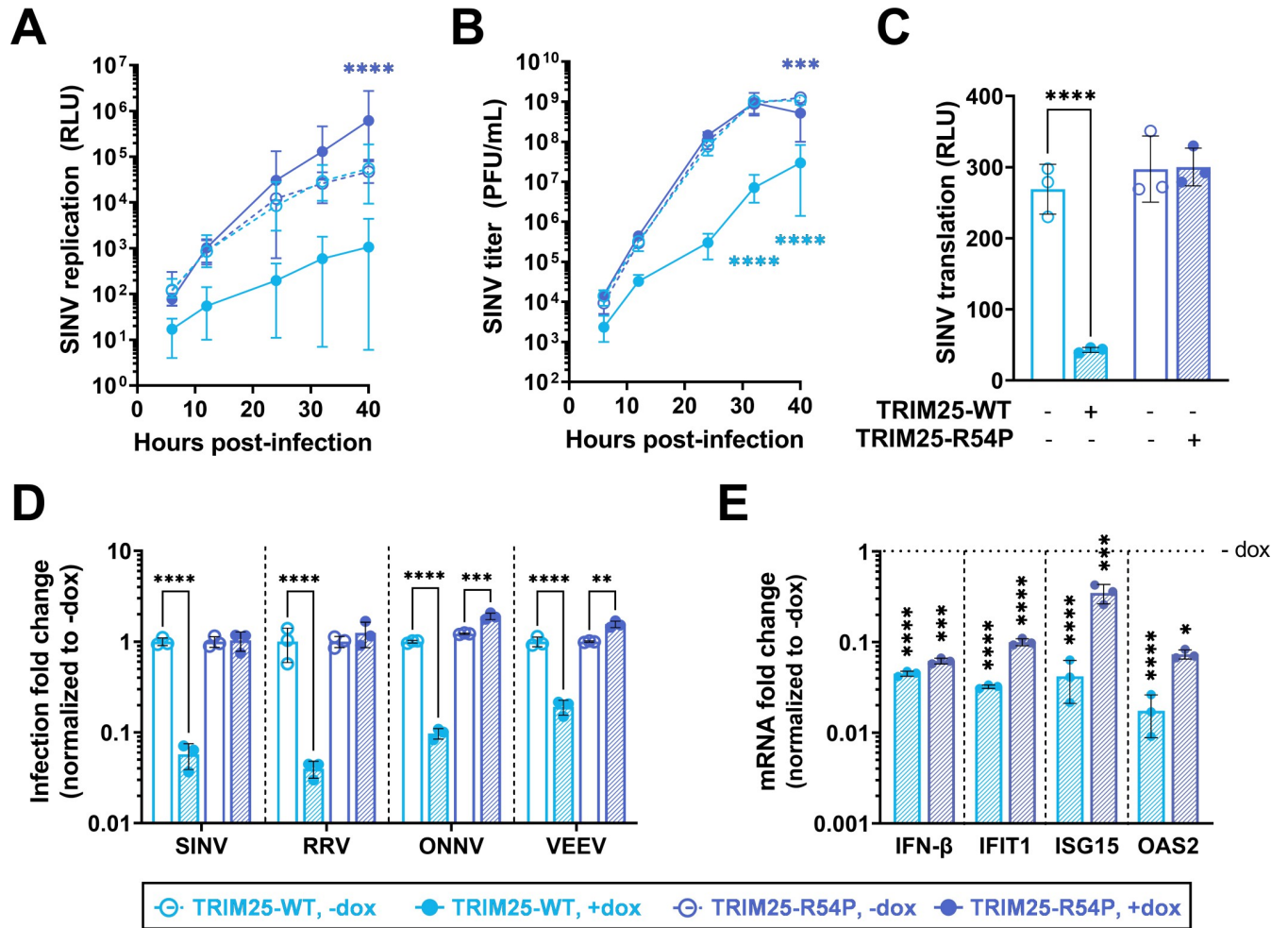
Fig 7. Point mutation in TRIM25 RING domain cripples TRIM25 antiviral activity. (A-C) Dox inducible TRIM25-WT or -R54P cells were induced for TRIM25-WT or -R54P expression at 1 μg/mL dox. Cells were infected with (A) SINV Toto1101/Luc at an MOI of 0.01 plaque forming unit (PFU)/cell, and lysed at 6, 12, 24, 32, and 40 hours post infection (h.p.i.); data combined from three independent experiments, error bars indicate range; or (B) Sindbis virus (SINV) Toto1101 at an MOI of 0.01 PFU/cell, harvesting supernatant at 6, 12, 24, 32, and 40 h.p.i. for plaque assays; data representative of two independent experiments, error bars indicate range; or (C) SINV Toto1101/Luc:ts6 at an MOI of 1 PFU/cell and lysed at 6 h.p.i. for measurement of luciferase activity; data representative of two independent experiments, error bars indicate standard deviation. (D) Percent infected cells (GFP+) at MOI of 0.01 PFU/cell (SINV 24 h.p.i.; Ross River virus (RRV) 24 h.p.i.; o'nyong-nyong virus (ONNV) 22 h.p.i.; Venezuelan equine encephalitis virus (VEEV) 10 h.p.i.) were normalized to that of the respective cell line without dox (set to one-fold). Asterisks indicate statistically significant differences, calculated using (A-B, D) Two-way ANOVA and Tukey's multiple comparisons test: **, p<0.01; ***, p<0.001; ****, p<0.0001; (light blue compares WT +/- dox, dark blue compares R54P +/- dox) or (C) Two-way ANOVA and Sidák's multiple comparisons test: ****, p<0.0001. Data for each virus (demarcated by dashed lines) was statistically analyzed independently. (E) TRIM25 inducible cells were treated with poly(I:C) in the presence or absence of dox, and RNA was harvested for RT-qPCR analysis. mRNA levels of IFN/ISGs in TRIM25-WT or R54P were normalized to that of the respective cell line without dox (set to one-fold, horizontal dotted line). Data representative of two independent experiments. mRNA fold change for each gene (demarcated by vertical dashed lines) was statistically analyzed independently. Asterisks indicate statistically significant differences as compared to the -dox condition (Two-way ANOVA and Sidák's multiple comparisons test: *, p<0.05; ***, p<0.001; ****, p<0.0001).
