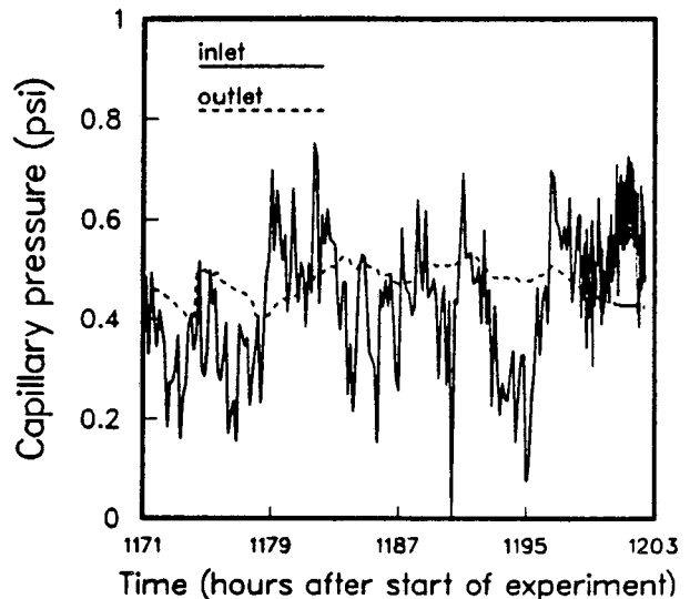
Figure 4. Inlet and outlet capillary pressures measured during steady state with q_{gas}/q_{liq} = 900 .
