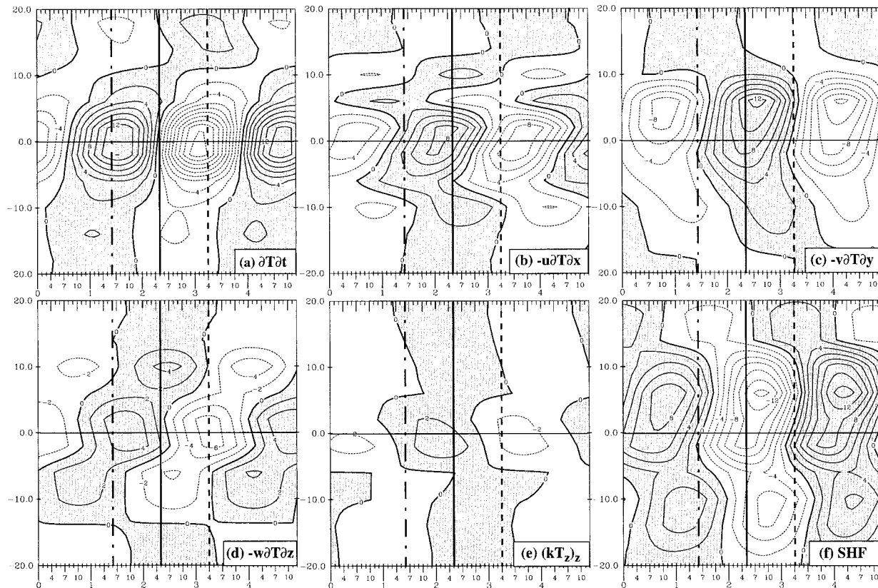
FIG. 14. Latitude–time structures of the budget terms for the upper-ocean layer during the simulated ENSO cycle. The structures are obtained from M-SSA analysis: (a) the time tendency term, (b) the zonal advection term, (c) the meridional advection term, (d) the vertical advection term, (e) the vertical diffusion term, and (f) the surface heat flux heating term. The onset, mature, and termination stage of the warm phase are indicated, respectively, by dot-dashed, solid, and dashed lines. Values shown are zonal averages and are amplified by 10 000. Contour intervals are 2^{\circ}\text{C day}^{-1} . Positive values are shaded.
