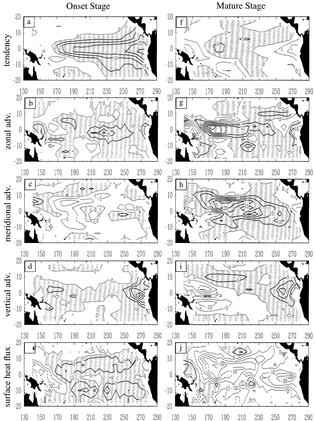
FIG. 15. Horizontal structures of the temperature budget terms for the upper ocean layer. The left panels show the structures at the onset stage of the warm phase, and the right panels are those for the mature stage. Values shown are amplified by 10 000. Contour intervals are 5^{\circ}\text{C day}^{-1} . Positive values are shaded.
