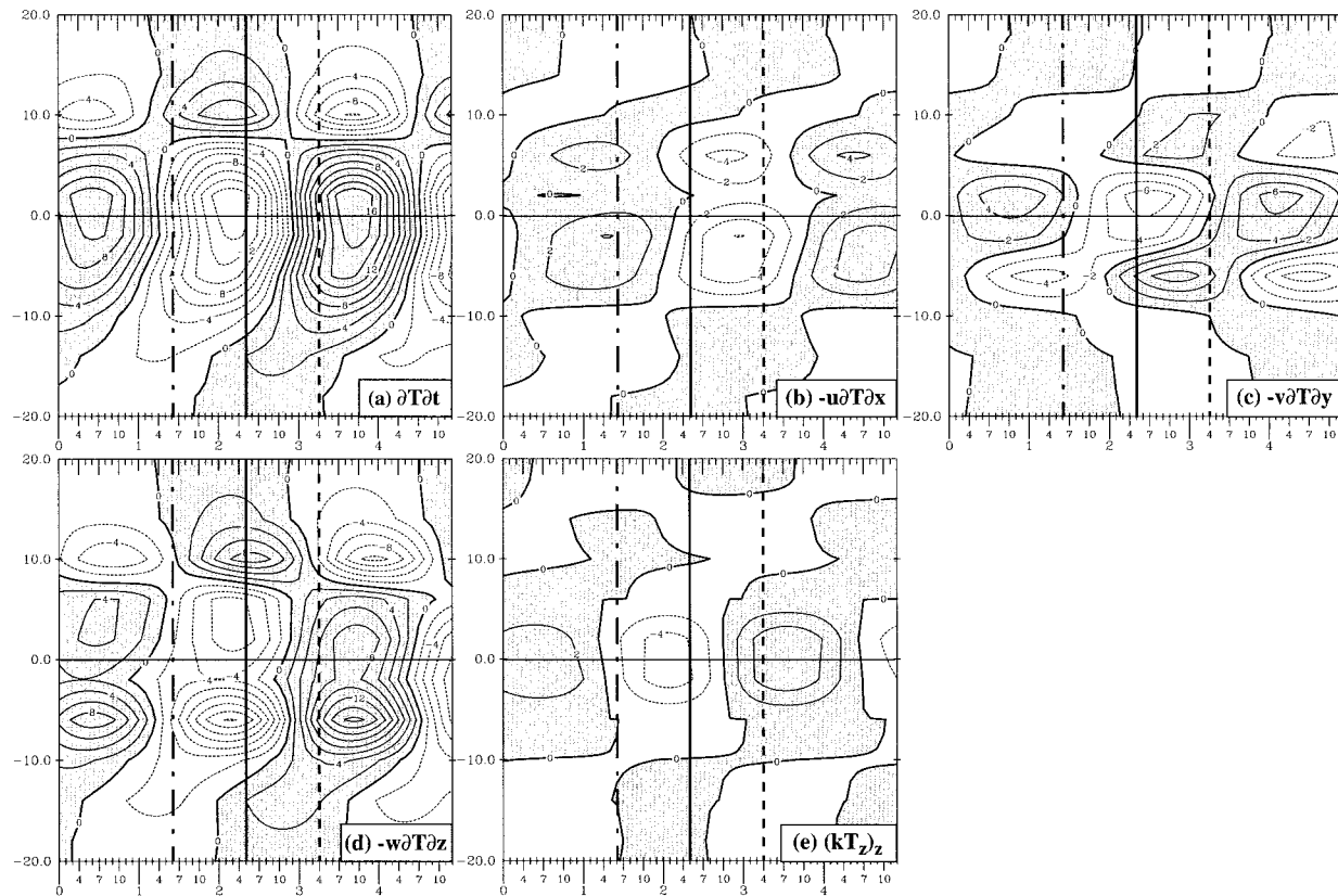
FIG. 17. Same as Fig. 14 but for the lower ocean layer and with the surface heat flux heating term omitted
