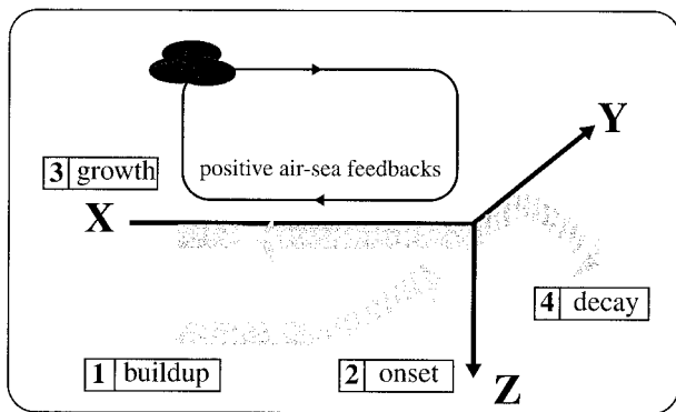
FIG. 13. A schematic of the four major movements of ocean temperature anomalies in the Pacific during the ENSO cycle. These processes include 1) buildup of a pool of surface temperature anomalies in the equatorial western Pacific, 2) a slow eastward and upward extension of the temperature anomalies from the western subsurface pool toward the surface of equatorial eastern Pacific during the onset stage, 3) a rapid amplification and slow westward expansion of SST anomalies on the ocean surface during the growing stage, and 4) the gradual northward and downward spread of temperature anomalies from the eastern equatorial Pacific toward the subsurface at 10^{\circ}\text{N} during the decaying stage. The positive air-sea feedback is considered part of the growing stage.
