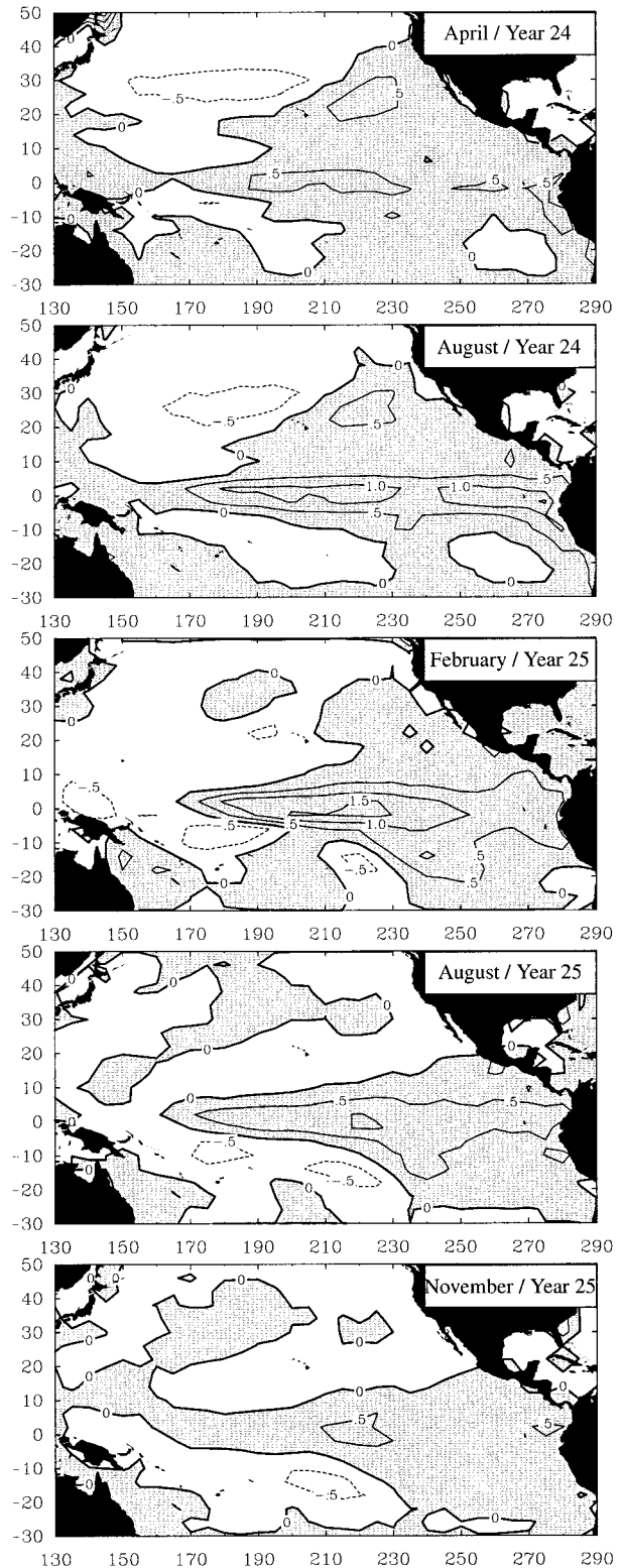
FIG. 3. Evolution of SST anomalies during the warm event in year 24 of the simulation. SST anomalies are obtained by removing the annual cycle and by filtering out variations with timescales shorter than 1 \text{ yr}^{-1} . Contour intervals are 0.5\text{°C} . Positive values are shaded.
