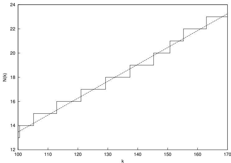
FIG. 2. The staircase function N(k) and the average staircase \bar{N}(k) . For the regular graphs the average staircase intersects every “stair” of the N(k) graph, with the separators (9) showing as the intersection points N(\bar{k}_n) = \bar{N}(\bar{k}_n) .
