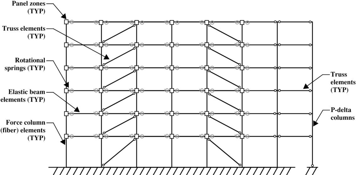
Figure 2-11: Elevation view of OpenSees model
