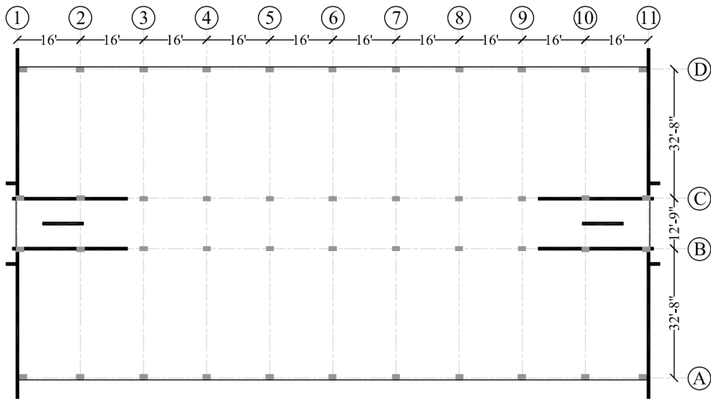
Figure 2-15 : Plan view of building at typical floor
