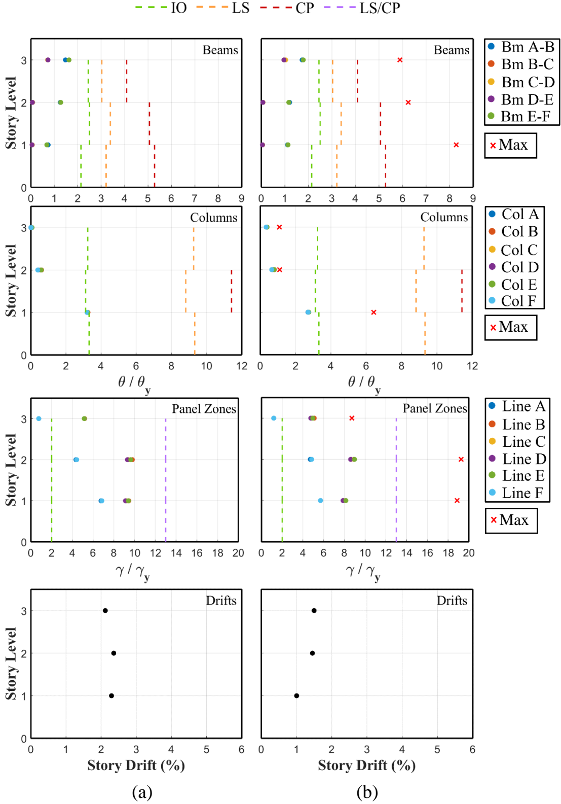
Figure 3-9: Inelastic demands in beams/columns/panel zones and interstory drifts from (a) Nonlinear Static Procedure and (b) Nonlinear Dynamic Procedure
