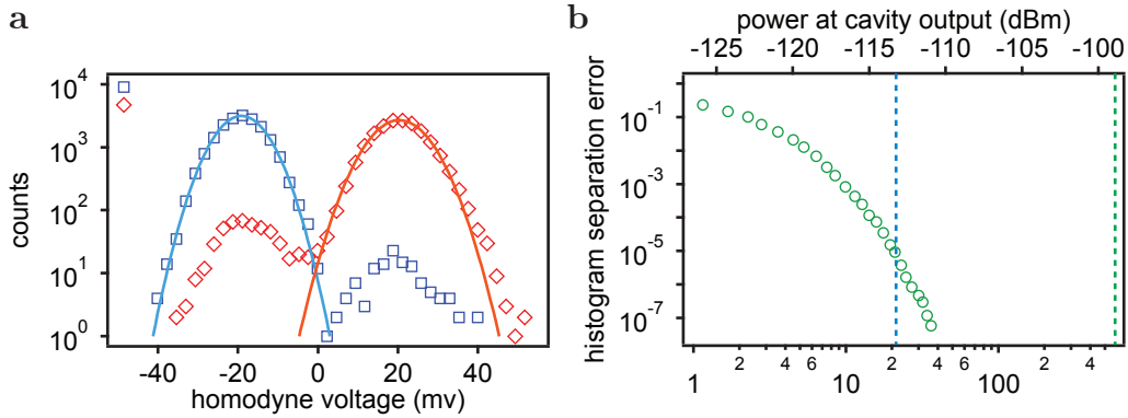
Figure 8.18: a Optimized projective readout histograms. The intrinsic overlap of the histograms contributes less than 10^{-5} of the total error. b Histogram separation error for 100 ns integration window. The measurement power required to achieve a histogram separation error below 10^{-5} (dashed blue line) is 14 dB below the measured 1 dB compression power of the JTWPA (dashed green line).
