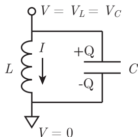
Figure 3.1: LC oscillator quantities and coordinates.
