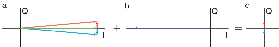
Figure 5.3: a IQ vector diagram showing the coherent state vectors for the ground state (pale blue) and excited state (pale red), and the decomposition of those vectors into the qubit state components (dark red and dark blue) and the component which contains no qubit state information (green), the dumb signal. b A coherent tone phase-shifted by 180 degrees with identical amplitude to the dumb signal. c The coherent addition of these vectors results in only the pure qubit state component without the large extra signal power associated with the dumb signal.
