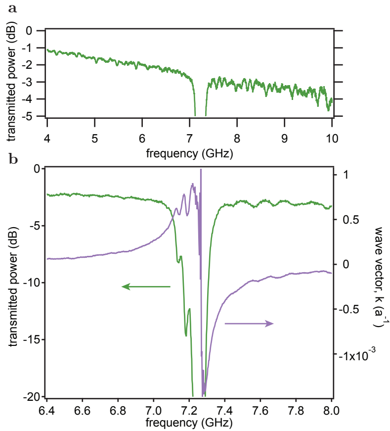
Figure 8.9: a Broadband small-signal power transmission, with axis scaled to clearly show the dielectric insertion loss of 1 to 4 dB. The transmission dip associated with the RPM resonators is visible just above 7 GHz. b Small-signal power transmission (green) and wavevector shift (purple) in the vicinity of the dispersion feature. The large linear component of the wavevector has been subtracted to show just the shift associated with the dispersion feature.
