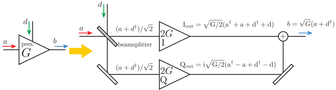
Figure 4.4: A schematic representation of how to create a phase-preserving amplifier with gain G as the combination of two phase-sensitive amplifiers with gain 2G and one beam splitter. We can physically understand the origin of the extra half-quantum of noise in this type of phase-preserving amplifier as the result of adding the second port on the beam splitter, introducing another vacuum mode d . Note that I have employed the large-gain limit to set \sqrt{G-1} = \sqrt{G} and eliminate the squeezed quadratures from the outputs of the phase-sensitive amplifiers.
