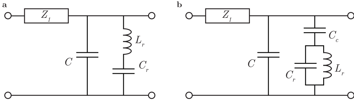
Figure 7.4: Shunt resonator topologies: a series LC shunt; b capacitively-coupled parallel LC shunt.
