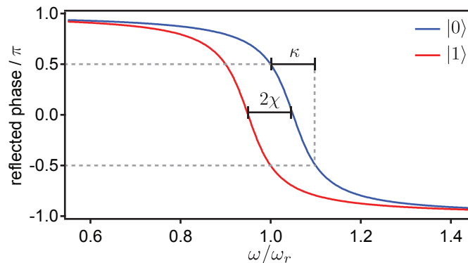
Figure 3.6: Reflected phase shift vs. normalized frequency for the case 2\chi = \kappa where \chi is negative. Measuring the phase of a reflected probe signal at a frequency where the reflected phase differs constitutes a measurement of the state of the qubit.
