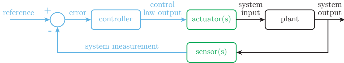
Figure 2.7: Block diagram of a generic feedback control system. The control portion of the system is drawn in blue, the interface between the control and the plant in green, and the plant itself in black.
