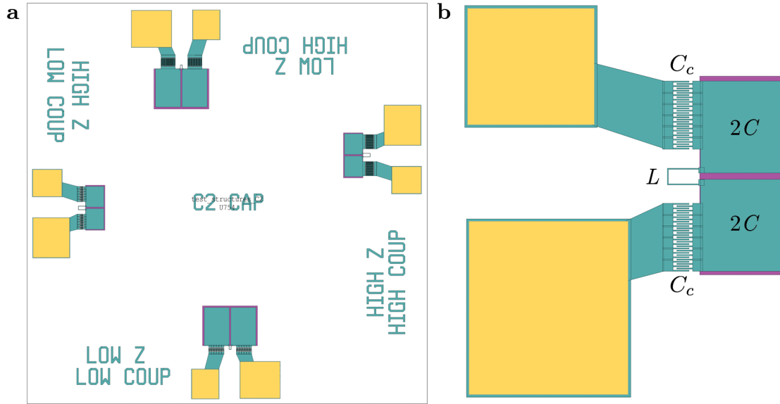
Figure 8.5: a Chip layout for C2 layer test resonators. b Close-up of the low-coupling, high-impedance test resonator from the left side of a .
