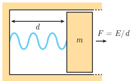
Figure 2.2: Apparatus for detecting the energy in a cavity resonator by measuring the ponderomotive force on a movable wall.
