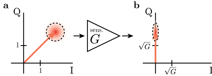
Figure 4.3: a IQ diagram of an input coherent state vector, including an uncertainty “blob” at the end of the vector representing the vacuum fluctuations. b The output state, following amplification by a phase-sensitive amplifier with gain G aligned with the Q quadrature (note axis rescaling). The action of the amplifier has amplified the input vector along the Q quadrature while de-amplifying the I quadrature. The resulting “squeezing” of the noise is visible in the shape of the noise blob, which has been stretched along Q by \sqrt{G} and compressed along I by 1/\sqrt{G} ; this compression along I implies the translation of the output state vector to the Q axis.
