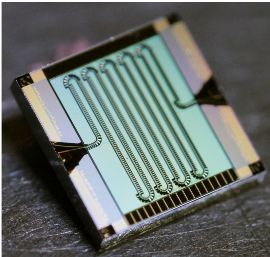
Figure 8.3: Macro photograph of a 2037 JJ RPM JTWPA. The chip is 5 mm \times 5 mm.
