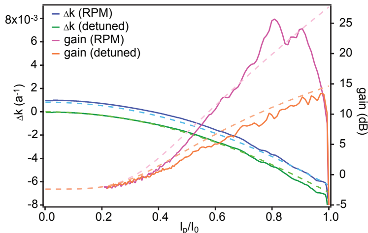
Figure 8.10: Total wavevector mismatch \Delta k (left axis) and corresponding amplifier gain (right axis) for a signal at 6.584 GHz. For the “RPM” traces, the pump was placed at 7.157 GHz, while the “detuned” traces have a pump at 6.5 GHz, far from the dispersion feature. Theory predictions are overlaid on the data as dashed lines in complementary colors. The total wavevector modification for the RPM case can be seen as the vertical offset on the left axis between the green and blue traces.
