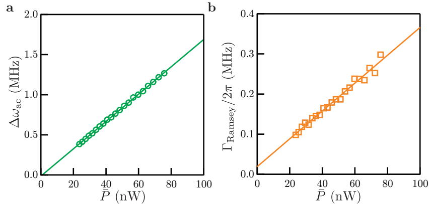
Figure 5.2: Measurements of AC Stark shift and measurement-induced dephasing rate vs. weak measurement power with linear fits. a Qubit frequency shift as a function of measurement power. Multiplying these values by the calibrated value for 2\chi results in the extracted value for \bar{n} as a function of input power. b Ramsey dephasing rate as a function of measurement power. The offset at zero measurement power corresponds to the total environmental dephasing rate (including non-idealities such as T_1 ).
