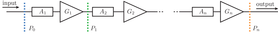
Figure 7.8: Block diagram of the model for distributed loss and gain, showing a series of discrete attenuators A_i each followed by a ideal phase-preserving amplifier with gain G_i .
