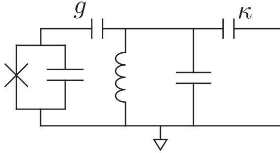
Figure 3.5: A circuit diagram which implements the same Hamiltonian as a cavity QED system. A transmon qubit, at left, is capacitively coupled with strength g to an LC resonator. The resonator is capacitively coupled to the environment with rate \kappa . It is also quite possible to replace one or both capacitive couplings with inductive couplings. The circuit as drawn contains an explicit ground reference, though this is not necessary and cQED systems are often implemented as partially or fully differential circuits to reject common-mode interference.
