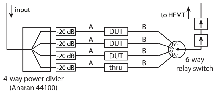
Figure 8.7: Microwave circuit schematic for cryogenic calibrated transmission measurements, using passive input multiplexing and active output multiplexing. Higher temperature stages not shown.
