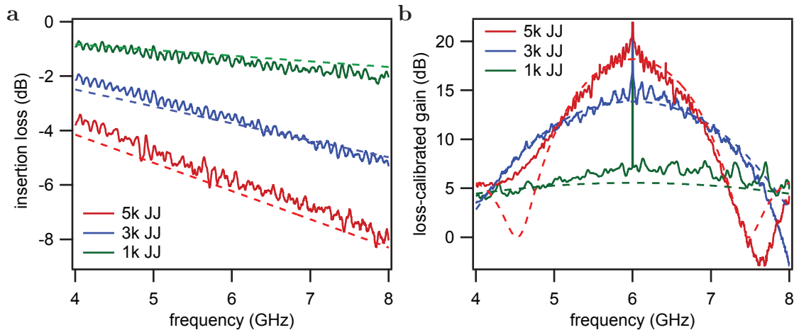
Figure 8.8: a Insertion loss for 1k, 3k, and 5k JJ devices, with theory predictions for a capacitor quality factor Q_i = 291 . b Measured gain profiles of 1k, 3k, and 5k JJ devices at identical pumping conditions ( \sim 0.75I_0 ), after subtracting the insertion loss measured in a , with theory overlays for the simple theory without loss.
