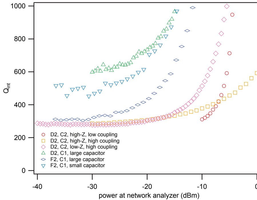
Figure 8.6: Measured internal quality factors for six test resonators, three from the C1 layer and three from C2. The traces have been offset on the power axis for clarity, to show the saturation in roughly the same regime.
