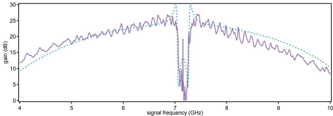
Figure 8.11: The gain profile measured with a pump at 7.157 GHz and a pump current of 91% of the critical current. A theory prediction for the measured device parameters, including the effects of loss for the signal and the pump, is overlaid as a blue dashed line.
