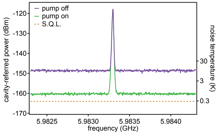
Figure 8.15: Calibrated output noise spectra. The spectrum taken with the pump on is referred to back to the input by subtracting the measured amplifier gain.
