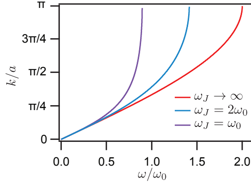
Figure 7.3: Dispersion relations for various ratios of plasma frequencies. The case where the inductance has no parallel capacitance is plotted in red. As the junction plasma frequency is reduced (finite shunt capacitance across the inductor), the cutoff frequency decreases and the curvature of the band increases.
