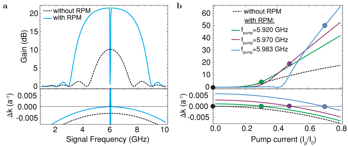
Figure 7.6: Gain of a 2000 unit cell JTWPA with and without RPM loading structures. a The gain as a function of signal frequency in dB with RPM (cyan) and without (black dashed) for a pump current of 0.5I_0 and a pump frequency of 5.97 GHz. The plot below shows the phase mismatch with RPM (cyan) and without (black dashed). The device with RPM is perfectly phase matched at zero detuning, and becomes poorly phase matched due to the curvature of the dispersion relation as the detuning is increased. b The peak gain as a function of pump current without RPM (black dashed) and with RPM for three different pump frequencies, which phase match the parametric amplification process for pump currents of 0.3 I_0 (green), 0.5 I_0 (purple), and 0.7 I_0 (cyan). The plot below shows the phase mismatch as a function of pump current. The dots mark the pump current where perfect phase matching is achieved. Adapted from reference [111].
