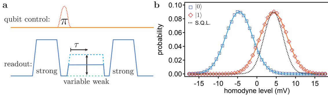
Figure 8.16: a Qubit and measurement pulse sequence. b Example weak measurement histograms with \bar{n} = 3.62 and \tau = 1 \mu\text{s} with gaussian fits. The black dashed line illustrates the histogram width expected for a fully quantum-limited measurement.
