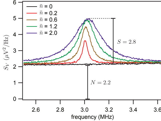
Figure 6.2: Measured CW Rabi spectra for several calibrated measurement powers, showing the saturation of the peak due to the measurement-disturbance tradeoff. The ratio of the peak height to the noise floor provides a measurement of the total measurement efficiency \eta .
