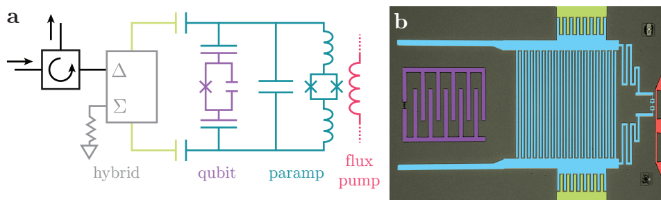
Figure 9.1: a Circuit model of transamp, showing differential launch using hybrid, single-junction transmon qubit in purple, nonlinear resonator (LJPA) in blue, and the bias line used to flux-pump the LJPA (red). b False-color electron-microscope image of a transamp chip; the coloring corresponds to the circuit schematic in a .
