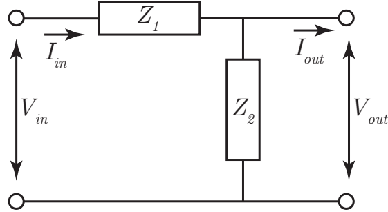
Figure 7.2: General two-port network under consideration, with one series impedance Z_1 and one shunt impedance Z_2 . Note current and voltage conventions.
