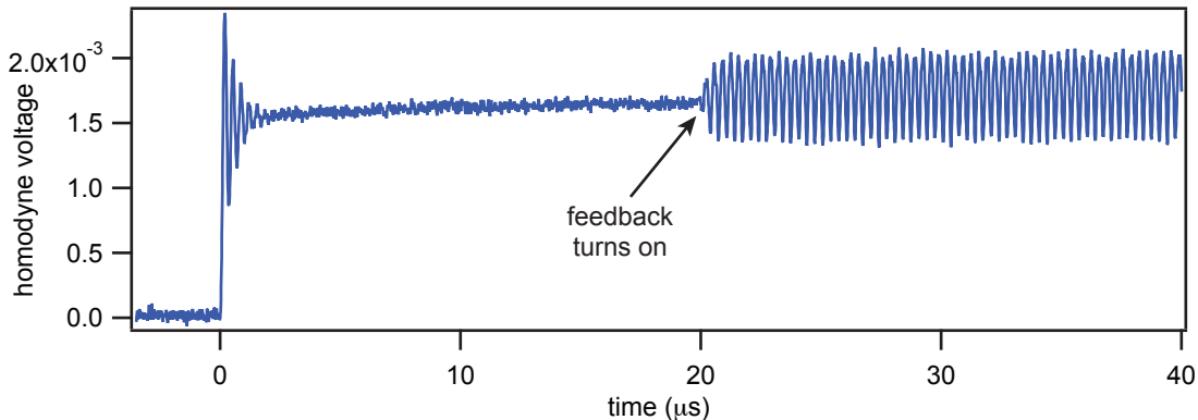
Figure 6.7: Time domain Rabi trace, showing the effect of delayed activation of the feedback control. The contrast is reduced compared to Figure 6.6b because this data was taken on a prior cooldown under different, less-optimized parameters.
