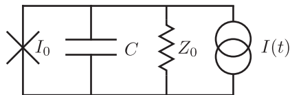
Figure 4.5: Circuit model for a Josephson nonlinear resonator operated as a LJPA. The nonlinear resonator is formed from the junction and capacitor at left, loaded by a transmission line modeled as a lumped impedance Z_0 and driven by an ideal current source I(t) .
