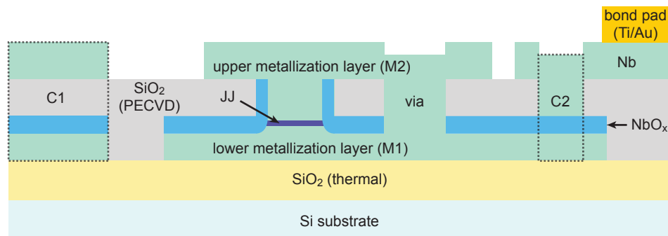
Figure 8.1: Schematic of the DSM process layers. Metal layers are 150 nm thick, the PECVD layer is 200 nm thick, and the \text{NbO}_x layer is 50 nm thick. Schematic is not shown to scale.
