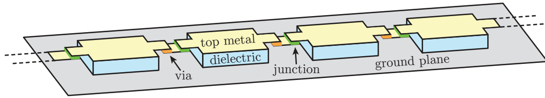
Figure 4.7: A quasi-microstrip geometry to realize a low-impedance JTWPA. The overall geometry looks something like a microstrip, with a center conductor (light yellow) situated on top of a ground plane (gray) with an intermediate dielectric layer (light blue). Here, the center conductor is periodically interrupted by a Josephson junction (green). A inter-layer via (orange) is used to make electrical contact with the bottom of the junction trilayer.
