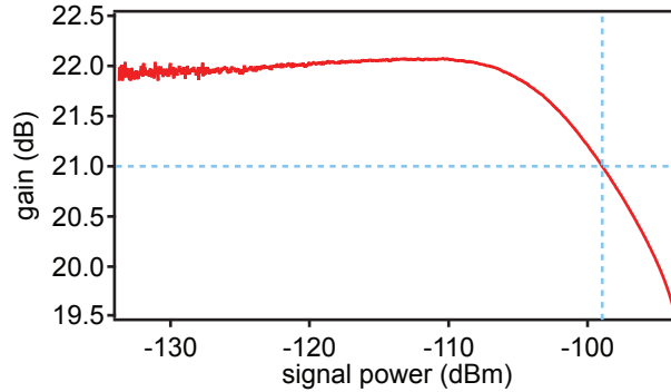
Figure 8.17: Measured input power gain compression curve, showing P_{1\text{dB}} = -99 dBm.
