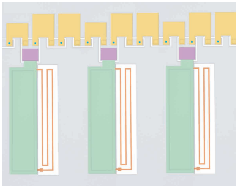
Figure 8.2: False-color optical micrograph of chip layout. M1 is shown as gray, with cutouts to form islands and accommodate the meander inductor. JJs are drawn in light blue. The top plate of the capacitance to ground is formed from M2 and colored yellow. The coupling capacitance to the resonator is formed from C1; the top plate (M2 layer) is colored purple. The resonator capacitance is formed from C2; the top plate (M2 layer) is colored green. The resonator meander inductor is colored orange; the via from M2 to M1 is the wider square at the bottom of the trace. The spacing between Josephson junctions is 16 \mu\text{m} .
