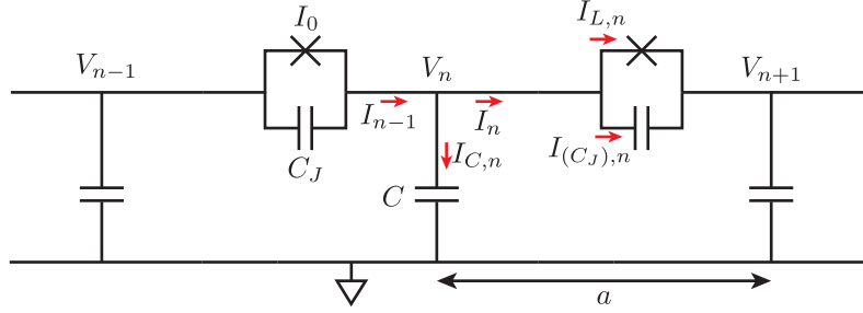
Figure 7.1: Circuit model for junction-loaded transmission line. The bottom wire is connected to ground, and the conventions for voltage drop and current flow are indicated.
