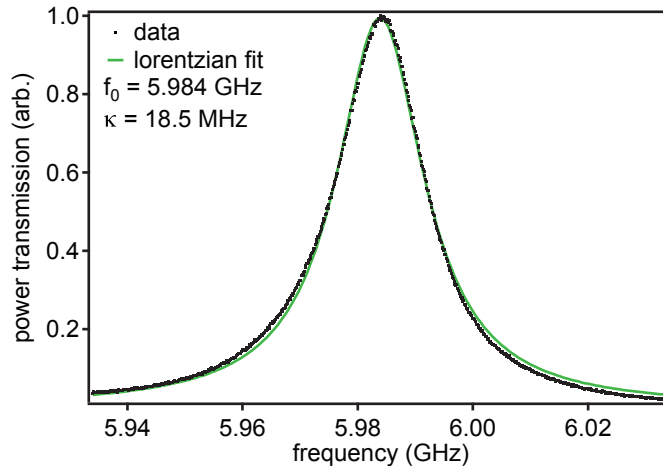
Figure 8.13: Lorentzian fit to cavity resonance. The measured cavity transmission spectrum deviates slightly from a perfect Lorentzian profile; we attribute this variation to transmission ripple in the microwave measurement chain, which is generally smooth but becomes significant on the order of 30 MHz.
