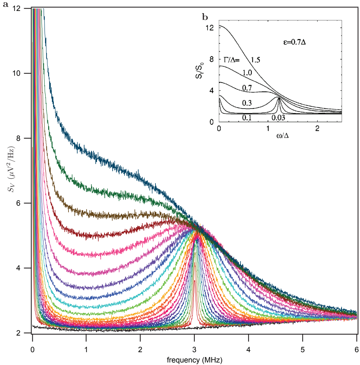
Figure 6.3: a CW Rabi traces taken over a broad range of measurement strengths, smoothly covering the evolution from lightly-perturbed oscillations to telegraph-like measurement pinning of the qubit state. b Theoretical curves for the same effect, showing beautiful qualitative agreement with the measured data. Note that the parameter regime in this theory plot is not the same as that for the experimental data. In fact the parameters in the plot are described in the language for a quantum dot qubit read out with a quantum point contact, though the physics for the two systems is identical in the relevant regime. Reproduced from reference [108].
