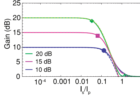
Figure 7.7: Amplifier gain as a function of input signal current, normalized to the pump current, for a small signal gain of 10, 15, and 20 dB obtained with a pump current of 0.5I_0 and device lengths of 1150, 1530, and 1900 unit cells. The approximation for the gain depletion (dashed lines) from (7.63) is in excellent agreement with the result obtained by solving the full nonlinear dynamics (solid lines). Adapted from reference [111].
