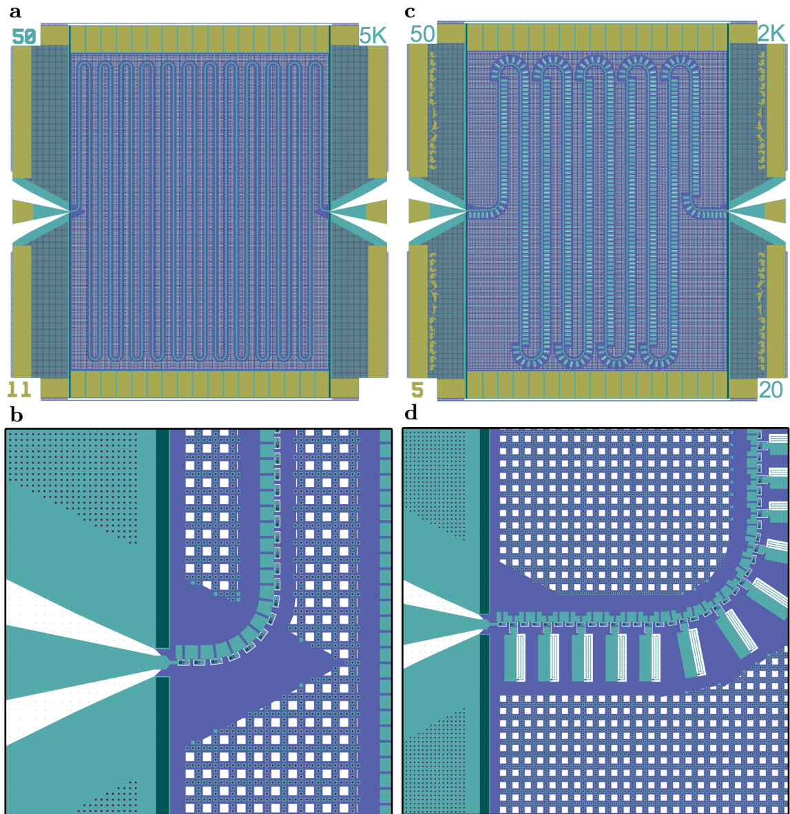
Figure 8.4: a Chip layout for 50\ \Omega 5022 JJ non-RPM device, from Reticle A. b Close-up of a , showing CPW-to-microstrip transition and nonlinear transmission line segment. c Chip layout for 50\ \Omega , 2037 JJ RPM device with 20 fF coupling capacitors, from Reticle B. d Close-up of c .
