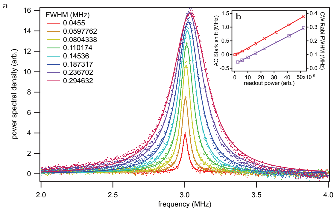
Figure 6.1: a CW Rabi spectra for a variety of measurement powers, from fairly weak measurement (red trace) to an optimal measurement power (magenta), and fits of the FWHM. At the highest measurement power we observe a saturation in the height of the peak with increasing measurement strength. This set of measurements was taken with a slightly odd paramp gain profile resulting in a sloping noise floor; this noise floor has been subtracted from the measured peaks for clarity and to improve the quality of the fits. b AC stark shift (from Ramsey measurements, not shown; plotted in red, left axis) and the FWHM dephasing from a (plotted in purple, right axis), showing the linear relationship with measurement power.
