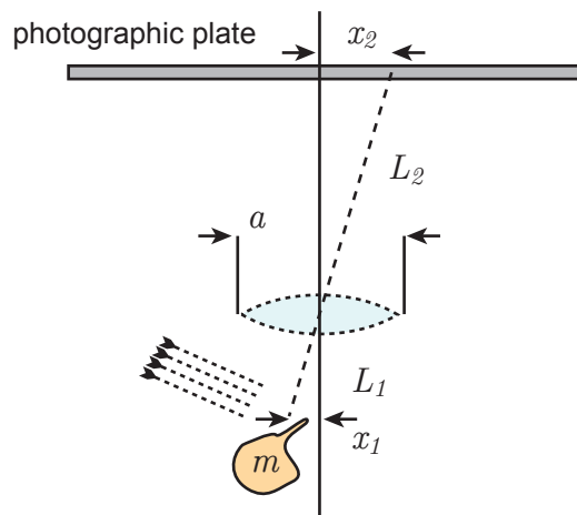
Figure 2.1: Heisenberg microscope apparatus.
