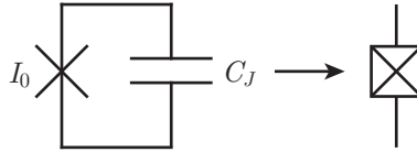
Figure 3.3: Circuit model for a Josephson junction including the intrinsic geometric parallel-plate capacitance. The symbol at right is the circuit symbol for a junction including its intrinsic capacitance.
