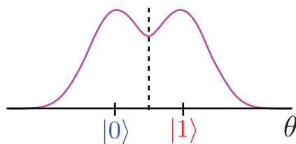
Figure 2.6: Histogram of the output of the classical meter for an ideal measurement of an ensemble of identically prepared qubit equal superposition states. The histogram overlap in this case is only due to fundamental quantum fluctuations of the measurement system, not added classical noise.
