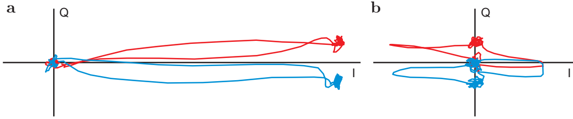
Figure 5.4: a Measured IQ trajectories for the ground state (blue) and excited state (red), showing the large dumb signal component. Axes have a square aspect ratio with arbitrary units. Trajectories start and end at the origin, so the loops correspond to the ring-up and ring-down of the resonator. b The same trajectories with the addition of the optimized dumb signal cancellation path. The separation at steady-state is the same, but the large extra signal power has been cancelled. Axes have the same scaling as in a .
