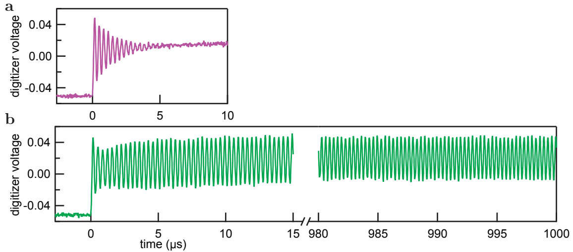
Figure 6.6: a A typical averaged time-domain Rabi oscillation, showing the characteristic exponential decay associated with dephasing. b Feedback-stabilized time domain Rabi oscillations. Adapted from reference [60].
