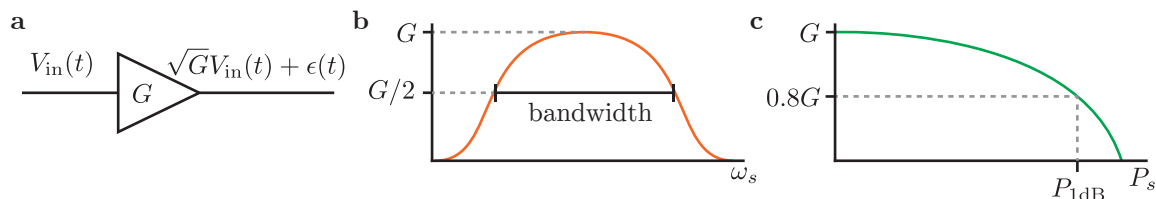
Figure 4.1: a A generic amplifier, characterized by its power gain G . The amplifier output contains an amplified copy of the signal as well as some additional noise \epsilon(t) . b The bandwidth of an amplifier is commonly defined as the frequency band over which the amplifier delivers a gain at least as large as G/2 . c The input signal power at which the gain is reduced to approximately 80% (-1 dB) of the small-signal gain is a common figure of merit for amplifier input power handling ability, called the 1 dB input compression power or P_{1\text{dB}} .
