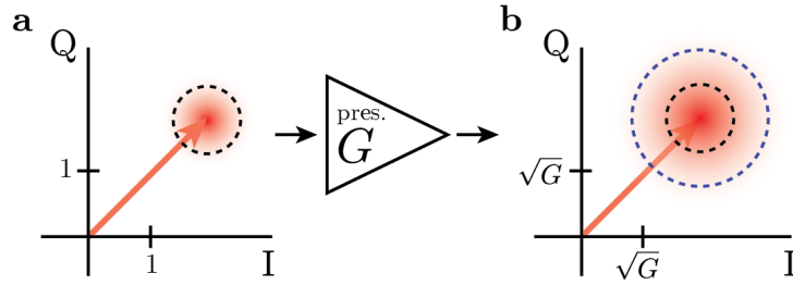
Figure 4.2: a IQ diagram of an input coherent state vector, including an uncertainty “blob” at the end of the vector representing the vacuum fluctuations. b The output state, following amplification by a phase-preserving amplifier with gain G (note axis rescaling). The action of the amplifier has amplified the input vector while maintaining the phase, but has also added some extra noise (dashed purple circle) onto the noise present at the input (black dashed circle).
