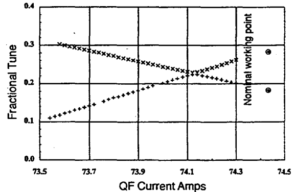
Figure 5. Tune variation observed through the coupling resonance.
