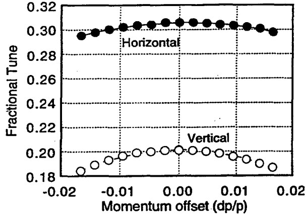
Figure 2. Variation of betatron tune with momentum.
