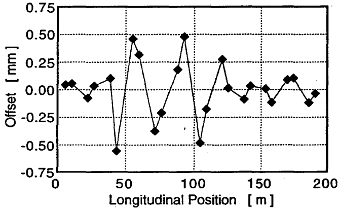
Figure 3. Horizontal offsets in SD sextupoles required to produce the \beta -beat shown in Figure 4.
