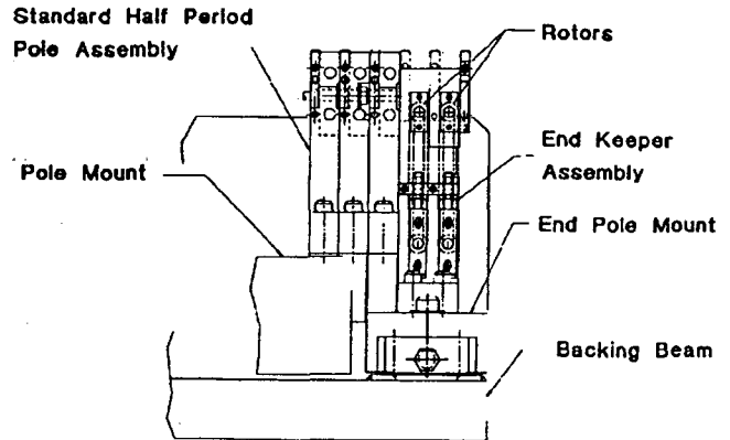
Fig. 3. End pole assembly.
