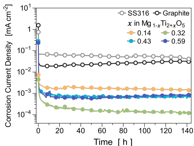
Figure 6. Development of the corrosion rate for MTOs with various compositions during 6 days of exposure in \text{H}_2\text{SO}_4 solution, \text{pH} = 1 .
