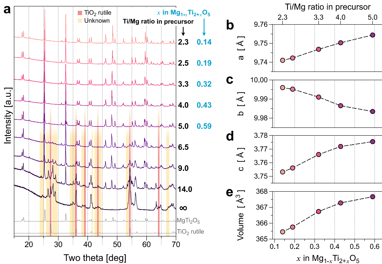
Figure 3. Series of XRD results of MTO synthesized from precursor with a TiO 2 content greater than Ti/Mg = 2.3. Note that the remaining TiO 2 rutile phase (indicated by the red box) appears in MTOs (Ti/Mg > 4.0) from the excessive Ti in the precursor. (b-e) Relations between the unit-cell parameters and volume as a function of x in Mg 1-x Ti 2+x O 5 .
