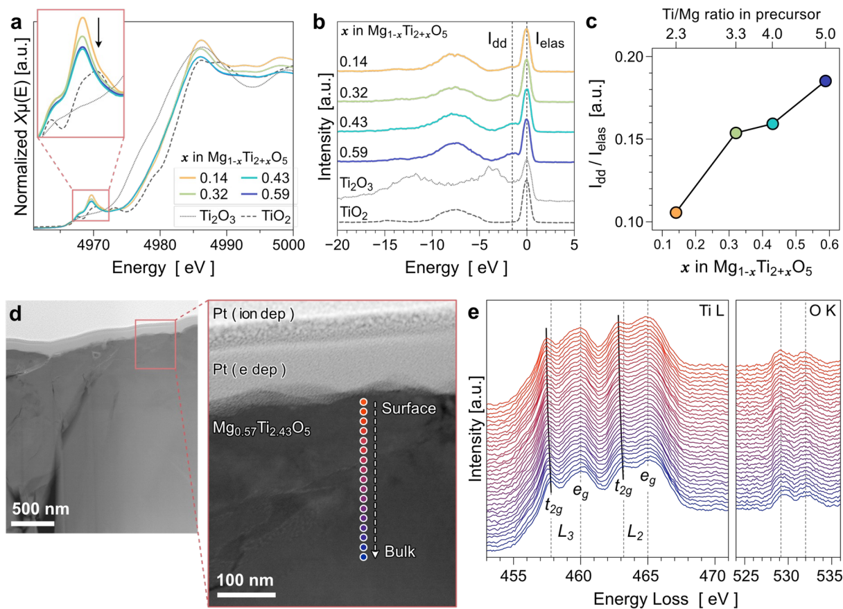
Figure 5. Chemical analysis of synthesized MTOs ( x = 0.14, 0.32, 0.43, and 0.59 in Mg_{1-x}Ti_{2+x}O_5 ). (a) Ti K-edge XANES results. The inset presents an enlarged view of the pre-edge region. (b) RIXS spectra collected with the excitation energy of 458 eV. Standard spectra of Ti^{3+}
