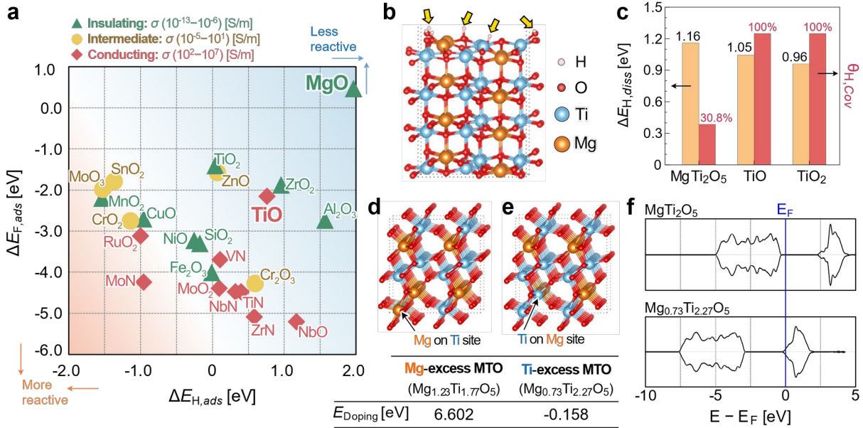
Figure 1. (a) Correlation observed between \Delta E_{H,ads} and \Delta E_{F,ads} after DFT single-adsorption calculations. (b) Hydrogen dissociation on a (110) MgTi_2O_5 slab model and (c) comparison of the hydrogen dissociation energy ( \Delta E_{H,diss} ) and hydrogen coverage ratio ( \theta_{H,Cov} ) of each Ti oxide. Note that only a few oxygen sites ( \sim 30.8\% ) showed hydrogen adsorption (denoted by the yellow arrows), suggesting MgTi_2O_5 is more protective in an acidic environment. Illustration of (d) Mg_{1.23}Ti_{1.77}O_5 and (e) Mg_{0.73}Ti_{2.27}O_5 structures, where an excessive Mg or Ti atom is occupying the Ti or Mg site in MgTi_2O_5 , respectively. The inset table presents a comparison of the doping energy of each model. (f) Total density of states (DOS) for MgTi_2O_5 and Mg_{0.73}Ti_{2.27}O_5 . Note that the Fermi level ( E_F ) of the Ti-excess MgTi_2O_5 system is occupied, in contrast to that of the stoichiometric MgTi_2O_5 .
