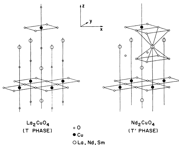
FIG. 1. Comparison of the T and T' crystal structures. For the T structure, the Cu ions are surrounded by oxygen octahedra, while for the T' structure, the Cu ions are fourfold coordinated to the oxygen ions in the plane.
