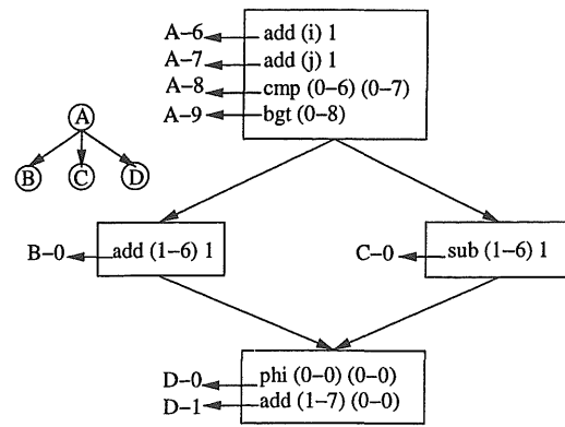
Figure 2: Reference-Safe Program in SSA Form
