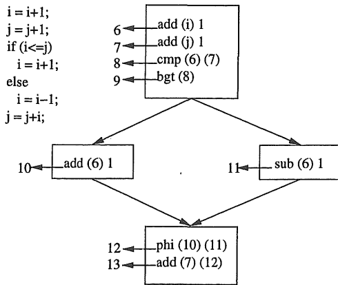
Figure 1: Program in SSA Form
