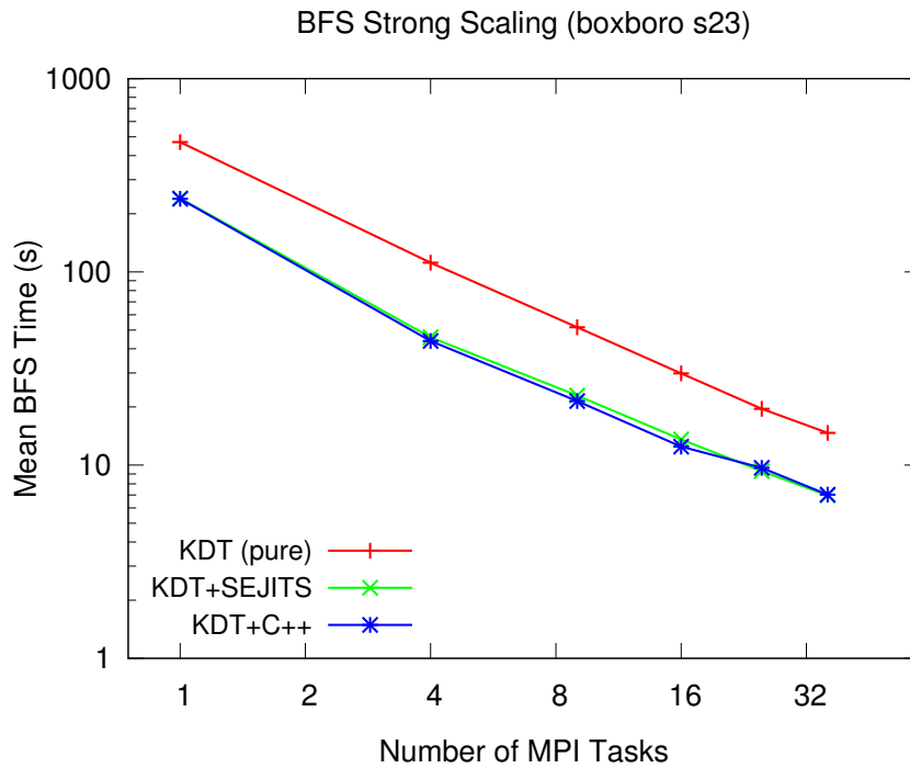
Figure 12.13: BFS strong scaling performance on Boxboro using three different semirings: KDT with pure Python semirings, KDT with our DSEL for semiring operations, and KDT using a semiring hand-coded in C++. The graphs are generated RMAT matrices using scale 22 (top) and scale 23 (bottom).
