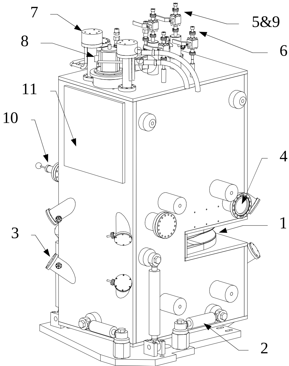
Fig. 8. Exterior configuration of the ALS Superbend: 1 - room temperature gap, 2 - suspension struts, 3 - cold mass suspension strap adjusters, 4 - cold mass fiducial viewports, 5 - LHe ports, 6 - LN 2 ports, 7 - current leads, 8 - cryocooler, 9 - rapid cooldown ports, 10 - rapid warmup feedthrough, 11 -access port.
