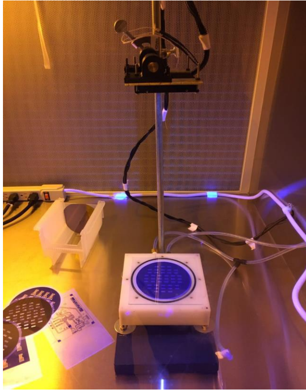
Figure 27: The expose step by using UV radiation
