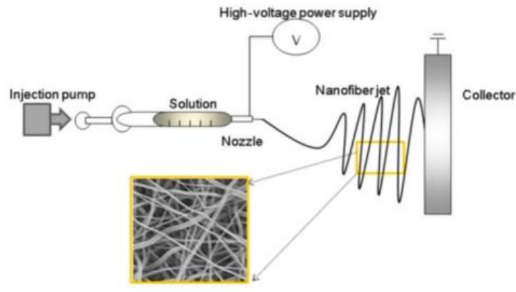
Figure 4: The schematic illustration of horizontal electrospinning setup.[19].
