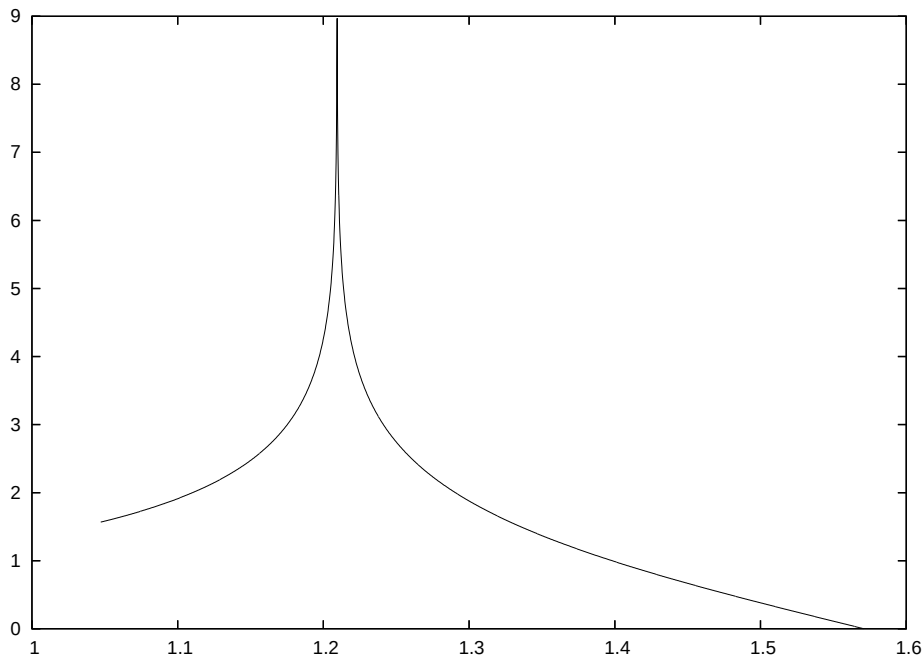
Figure 1: Integrand function with singularity
