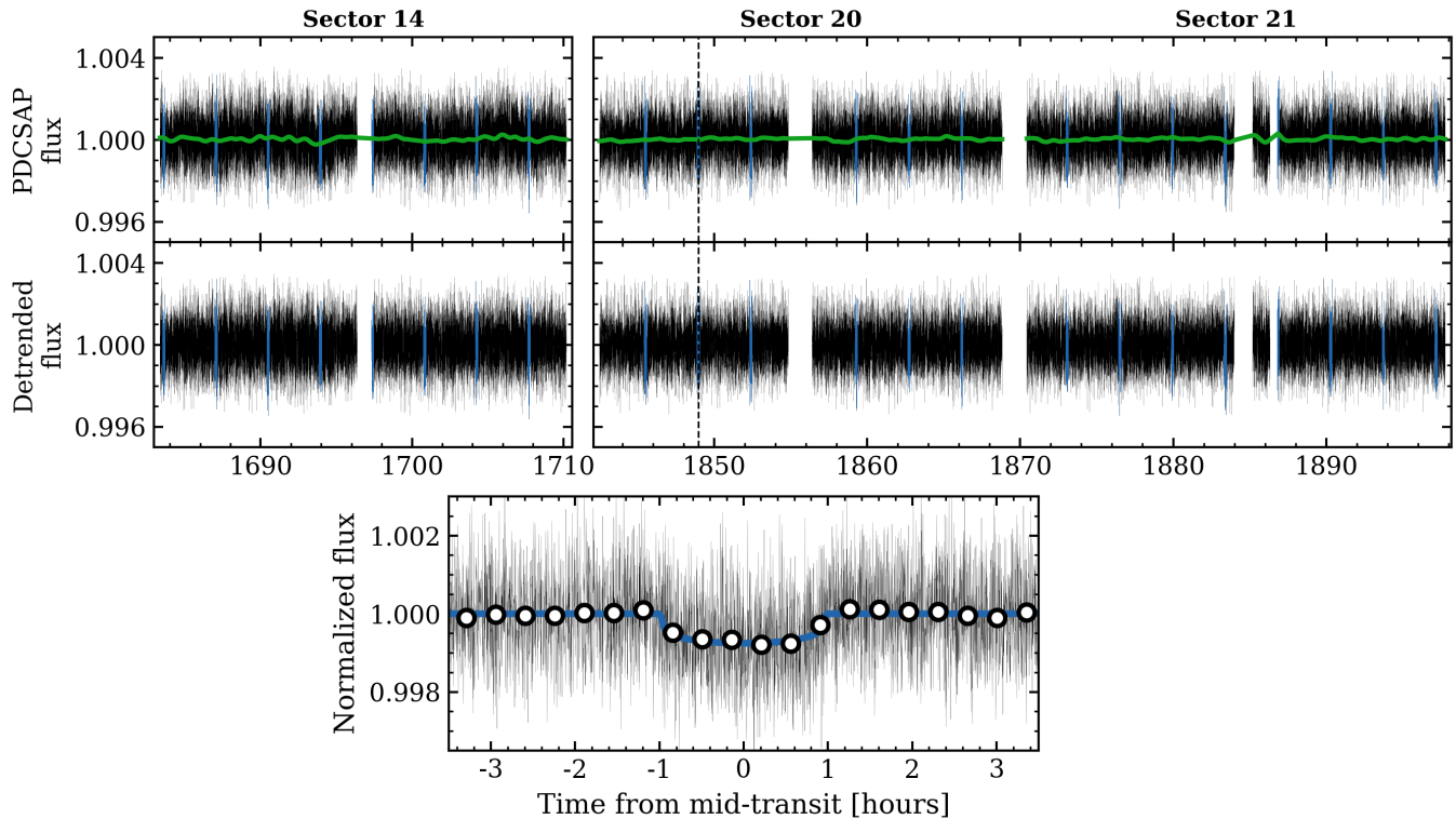
Figure 2. TESS light curve of TOI-1235 from sectors 14, 20, and 21. Upper row: the PDCSAP light curve following the removal of systematics via a linear combination of Cotrending Basis Vectors. The green curve depicts the mean GP model of residual temporally correlated noise (Sect. 4.1). The 3\sigma uncertainties on the mean GP model are smaller than the curve width. In-transit measurements are highlighted in blue throughout. The vertical dashed line highlights the epoch of the ground-based transit observation from LCOGT, which confirms the transit event on-target (Sect. 3.4). Lower row: the detrended PDCSAP light curve. Bottom panel: the phase-folded transit light curve of TOI-1235 b from 22 individual transit events. The maximum a-posteriori transit model is depicted by the blue curve while the white markers depict the binned photometry.
