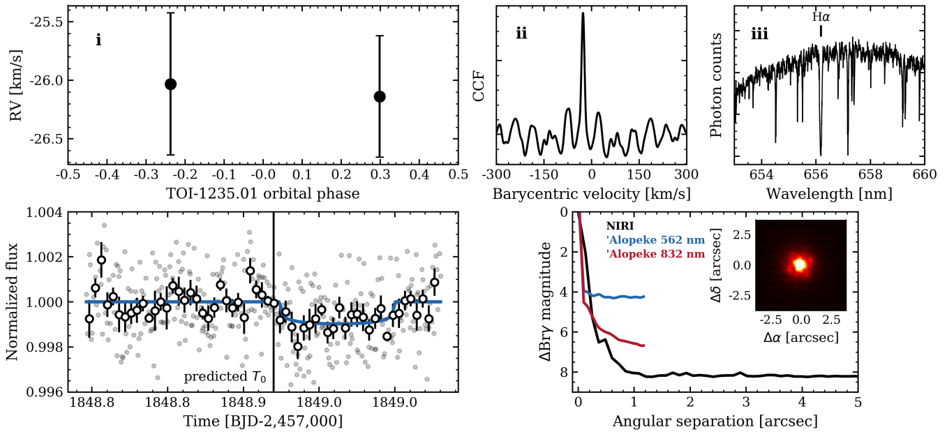
Figure 4. Summary of TFOF follow-up observations of TOI-1235 for planet validation purposes. Top row: results from TRES reconnaissance spectroscopy that i) show no RV variations thus ruling out a spectroscopic binary, ii) reveal a single-lined CCF with no rotational broadening, and iii) show H\alpha in absorption. Lower left panel: the ground-based transit light curve obtained with LCOGT showing that the expected transit event occurred on-target and arrived 63 minutes late relative to the SPOC-reported linear ephemeris represented by the black vertical line . Open circles depict the light curve in 5.5 minute bins. The blue curve depicts the optimized transit fit to the LCOGT photometry. Lower right panel: the 5\sigma contrast curves from Gemini/NIRI AO-imaging ( black ), ‘Alopeke 562 nm speckle imaging ( blue ), and ‘Alopeke 832 nm speckle imaging ( red ). The inset depicts the coadded image from Gemini/NIRI AO-imaging centered on TOI-1235.
