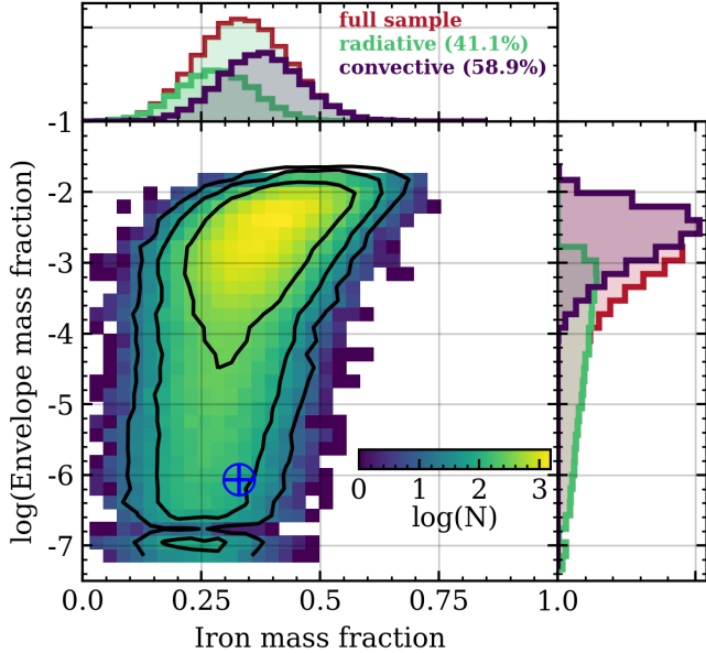
Figure 7. Joint distribution of TOI-1235 b’s iron mass and envelope mass fractions to be consistent with its measured mass and radius. The colormap represents the number of successful planet models given X_{\text{env}} and X_{\text{Fe}} while the contours highlight the 68, 95, and 99 percentiles. The top and right 1D histograms depict the marginalized distributions of X_{\text{Fe}} and \log_{10}(X_{\text{env}}) respectively for the full sample (red), plus the subset of realizations with a radiative atmospheres (green) and convective atmospheres (blue). The blue cross highlights the Earth.
