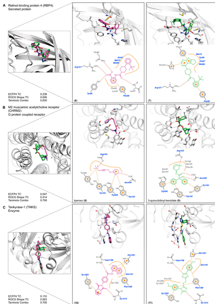
Figure 3. Examples of class I complexes, where the same protein residues interact with different ligand functional groups (see Table SI-1 and Figure SI-4 in the Supporting Information). The structure overlap, binding site of each complex, 2D outline of protein–ligand interactions (blue dots are water, red dashed lines hydrogen bonds, orange lines represent hydrophobic contact; blue residue labels are common to both), and similarity metrics are shown. (A) Retinol-binding protein 4 bound to compound 6 and to compound 7. (B) M 2 muscarinic receptor bound to Iperoxo (8) and to QNB (9). (C) Tankyrase-1 bound to compounds 10 and 11.
