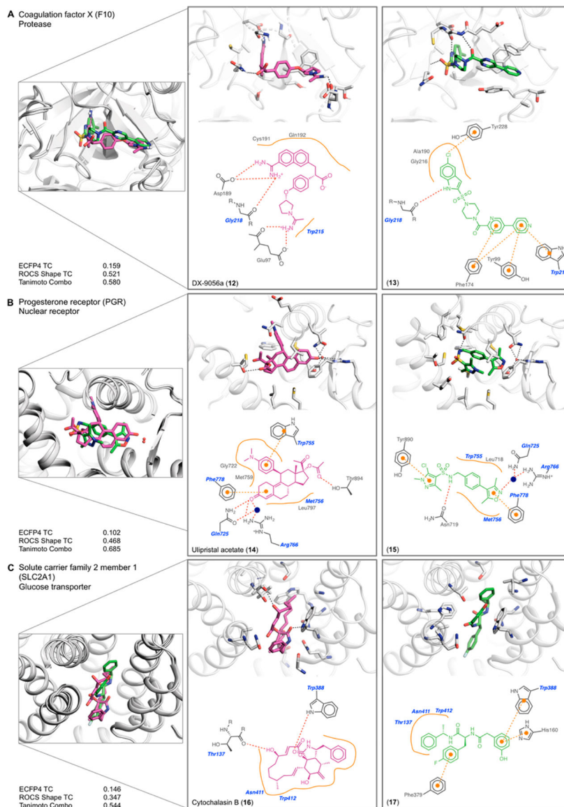
Figure 4. Examples of class II complexes where different protein residues engage different ligand functional groups (see Table SI-2 and Figure SI-5 in the Supporting Information). The 3D crystal structure overlap, enlarged binding site of each complex, 2D outline of protein–ligand interactions (colored as in Figure 3), and similarity metrics are shown. (A) Coagulation factor Xa bound to DX-9056a ( 12 ) and to compound 13 . (B) Progesterone receptor bound to ulipristal acetate ( 14 ) and to compound 15 . (C) Glucose transporter bound to cytochalasin B ( 16 ) and to compound 17 .
