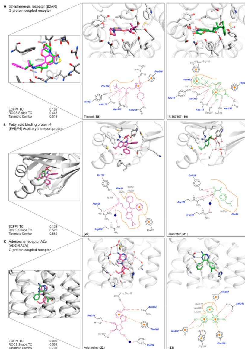
Figure 5. Examples of class III complexes where the same protein residues interact with similar functional groups on the ligands (also see Table SI-3 and SI-6). The structure overlap, enlarged binding site of each complex, 2D outline of protein–ligand interactions (colored as in Figure 3), and similarity metrics are shown: (A) \beta_2 -adrenergic receptor bound to timolol (18) and to BI167107 (19); (B) FABP4 bound to compound 20 and to ibuprofen (21); and (C) adenosine receptor A2a bound to adenosine (22) and to compound 23.
