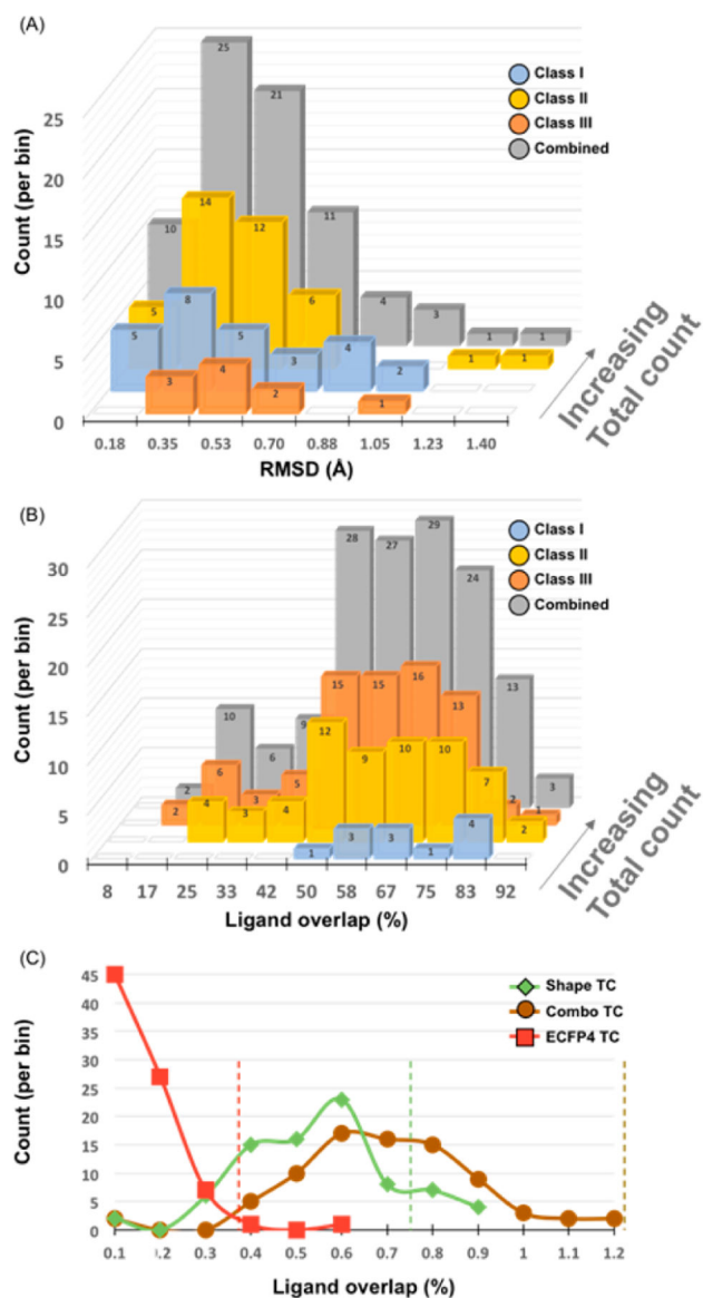
Figure 2. Statistics for binding site residue overlap, ligand volume overlap, and ligand similarity for the 76 complex pairs. (A) Binding site residue overlap (all heavy atoms) of complex pairs in each of the three classes and totaled overall. (B) Ligand volume overlap in each complex pair, separated by class and summed overall. Most pairs contain one ligand with 50% of its volume overlapped, indicating ligands are in the same binding pocket. (C) Dissimilarity of ligands in complex pairs for all three classes, by three different metrics: ECFP4 fingerprints, ROCS shape, and ROCS TanimotoCombo. Most are below common values used to distinguish chemically dissimilar scaffolds (dashed lines with corresponding colors).
