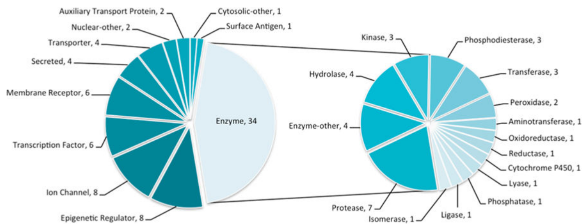
Figure 1. Protein families represented in this study. (Left) Distribution of major drug-relevant protein families within the 76 proteins considered (count after the comma). (Right) Distribution of enzyme subfamilies. All family names are ChEMBL target classifications. 18
