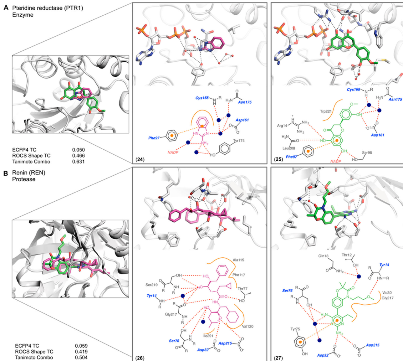
Figure 6. Complex pairs where water mediates interactions with one ligand whereas the second ligand makes these interactions directly. The structure overlap, binding site of each complex, 2D outline of protein–ligand interactions (colored as in Figure 3), and similarity metrics are shown. (A) Pteridine reductase co-crystallized with compound 24 and with compound 25 . (B) Renin co-crystallized with compound 26 and with compound 27 .
