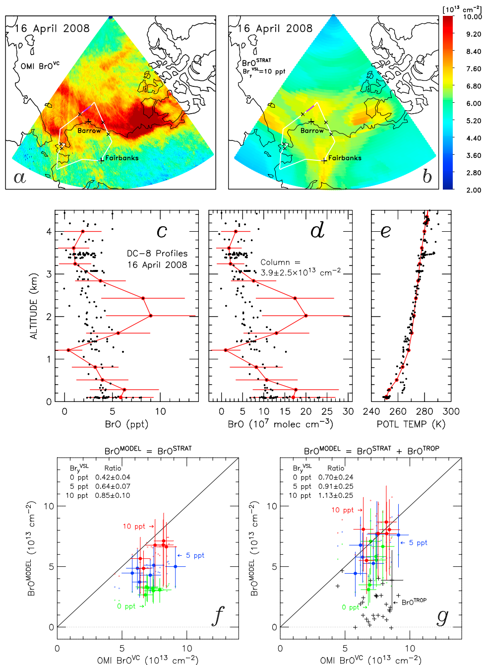
Figure 4. (a and b) Flight track of the DC-8 on 16 April 2008 (white line) superimposed on OMI measurements of \text{BrO}^{\text{VC}} and calculated \text{BrO}^{\text{STRAT}} ( \text{Br}_y^{\text{VSL}} = 10 \text{ ppt} ), respectively. (c–e) Profiles of BrO volume mixing ratio, BrO concentration, and potential temperature ( \theta ) on 16 April 2008 (black dots); profile shown in red, with \text{BrO}^{\text{TROP}} = 3.9 \pm 2.5 \times 10^{13} \text{ cm}^{-2} , was measured at the segment marked in purple in Figures 4a and 4b; \times denotes location of other profiles. All data were acquired for \text{O}_3 < 120 \text{ ppb} , assuring the sampling of tropospheric air. (f and g) Scatter plot of \text{BrO}^{\text{MODEL}} versus OMI \text{BrO}^{\text{VC}} for locations of the DC-8 and WP-3D measurements of \text{BrO}^{\text{TROP}} , where \text{BrO}^{\text{MODEL}} = \text{BrO}^{\text{STRAT}} (Figure 4f) and \text{BrO}^{\text{MODEL}} = \text{BrO}^{\text{STRAT}} + \text{BrO}^{\text{TROP}} (Figure 4g), for values of \text{Br}_y^{\text{VSL}} from the 0, 5, and 10 ppt simulations. Determinations of \text{BrO}^{\text{TROP}} (+) are shown in Figure 4g. Error bars for OMI \text{BrO}^{\text{VC}} represent 1\sigma uncertainty due to residuals in the spectral fit. Error bars for \text{BrO}^{\text{MODEL}} represent 1\sigma uncertainty in \text{BrO}^{\text{STRAT}} (Figure 4f) and RSS combination of 1\sigma uncertainty in \text{BrO}^{\text{STRAT}} and \text{BrO}^{\text{TROP}} (Figure 4g). For clarity, error bars are shown for every 5th data point and just one measurement of \text{BrO}^{\text{TROP}} . Values of the ratio \text{BrO}^{\text{MODEL}}/\text{OMI BrO}^{\text{VC}} are indicated on Figures 4f and 4g.
