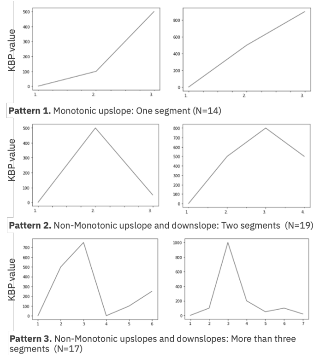
Figure 3: Examples of three different patterns (x-axis: n^{\text{th}} attempt; y-axis: the attempted KBP values). For example, the sequence of attempted KBP values in the first graph is 0, 100, 500.
