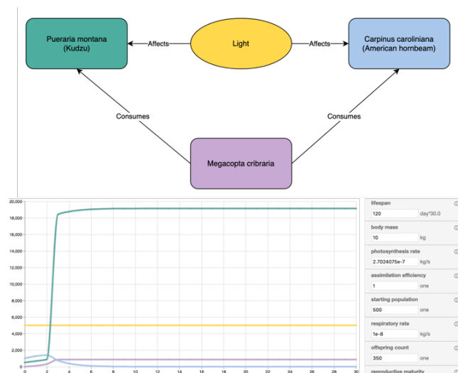
Figure 1: The conceptual model, the simulation parameters of kudzu, and the simulation output generated based on the conceptual model and its parameters. X axis: Time (months). Y axis: Population. The color of lines represents the biotic and abiotic components in the conceptual model.
