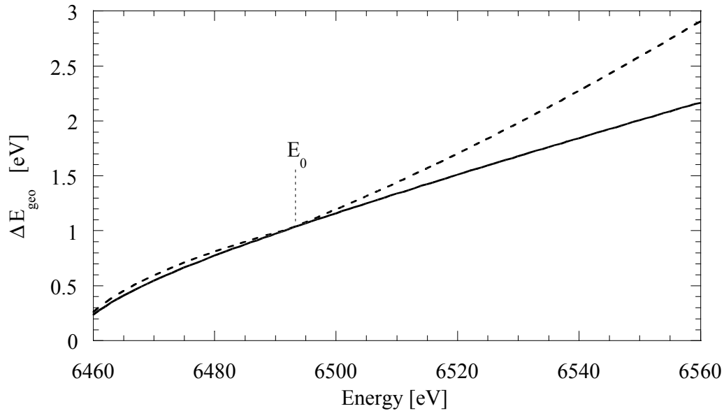
Figure 3 Calculated energy resolution for a long scan at the Mn K\beta emission with (dashed line) and without (solid line) contributions resulting from the deviation of the Rowland condition in a vertical scan. The source size is set to \delta x = \delta y = 5\text{mm} , \delta z = 1.0\text{mm} .
