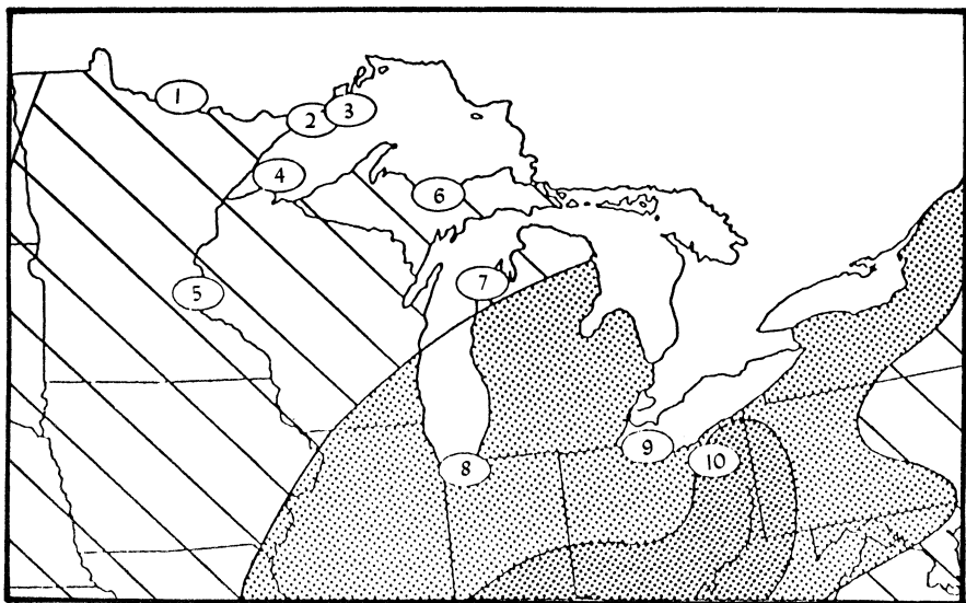
Figure 1. Visual range ( V ) isopleths for non-urban areas, 1974-76. Visual range in northwestern Minnesota falls between 25 and 45 miles. Modified from Trijonis and Shapland (1979). Locations of park areas—1: Voyageurs; 2: Grand Portage; 3: Isle Royale; 4: Apostle Islands; 5: St. Croix; 6: Pictured Rocks; 7: Sleeping Bear Dunes; 8: Indiana Dunes; 9: Perry's Victory; 10: Cuyahoga Valley.
