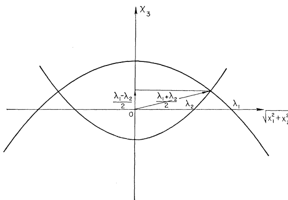
FIG. 3. Parabolic coordinates.
