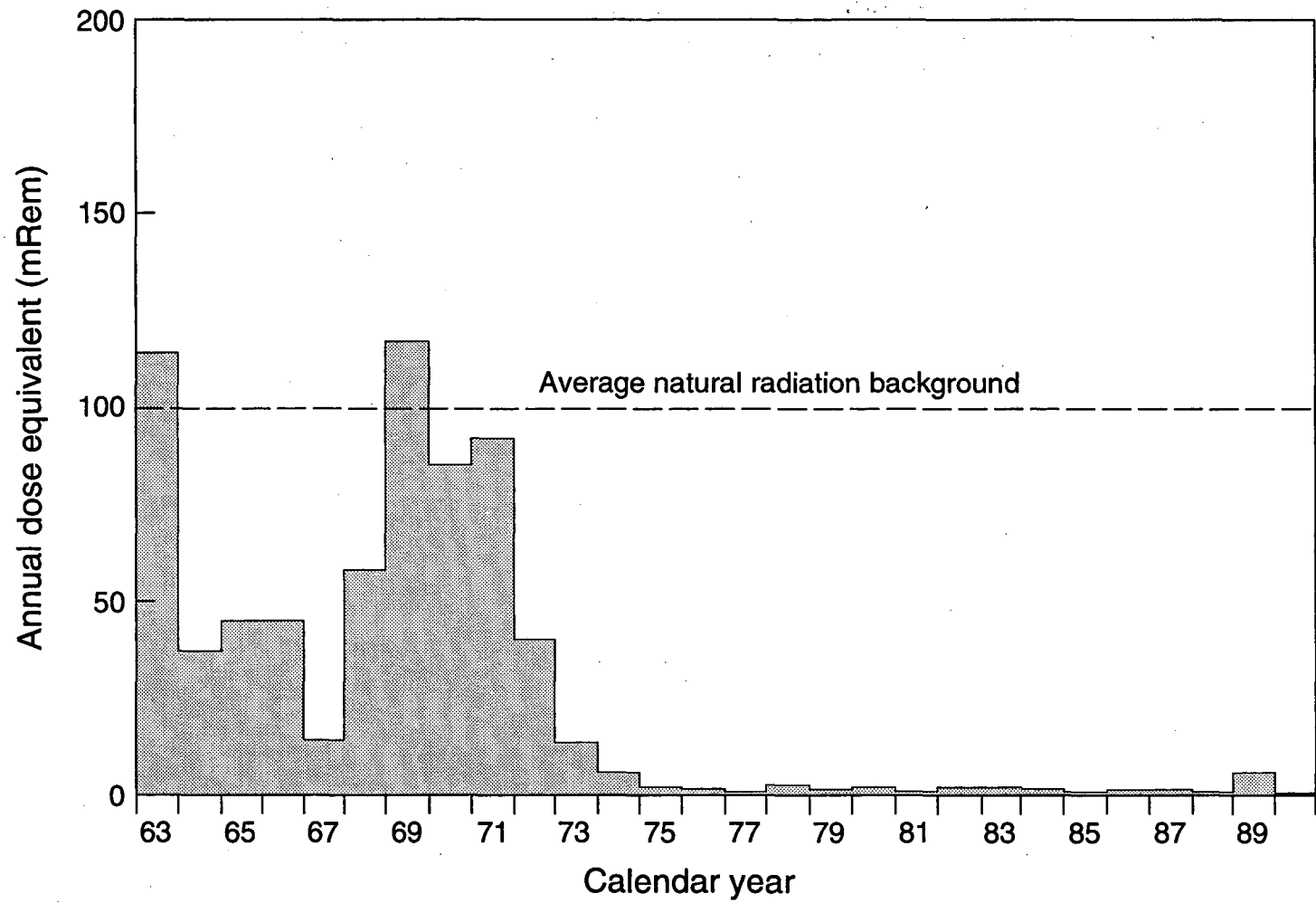
Figure 9. Annual accelerator-produced dose equivalent at Building 90 Environmental Monitoring Station, 1962-1990.
