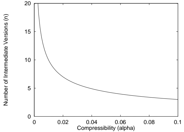
(b) Number of intermediate versions at minimum of s(n) .
