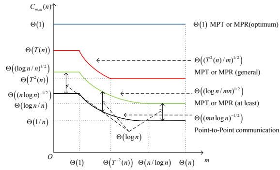
Fig. 3. Order throughput capacity of (n, m, m) -cast with MPT or MPR and point-to-point communication as a function of number of destinations m and transceiver range T(n)
