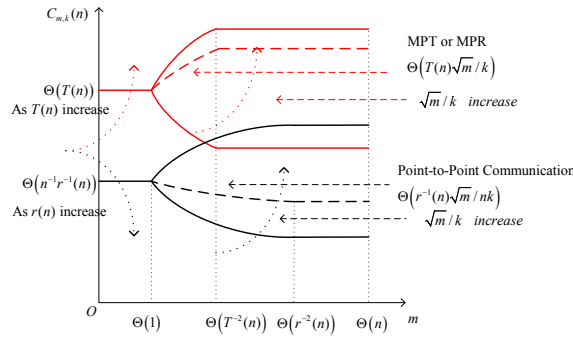
Fig. 4. Order throughput capacity of (n, m, k) -cast with MPT or MPR and point-to-point communication
