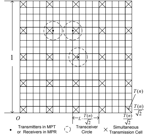
Fig. 2. Cell construction used to derive a lower bound on capacity
