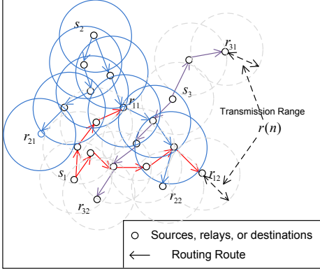
Fig. 1. Illustration of three (n, m, k) -cast trees in a network of 22 nodes when m = k = 2 .
