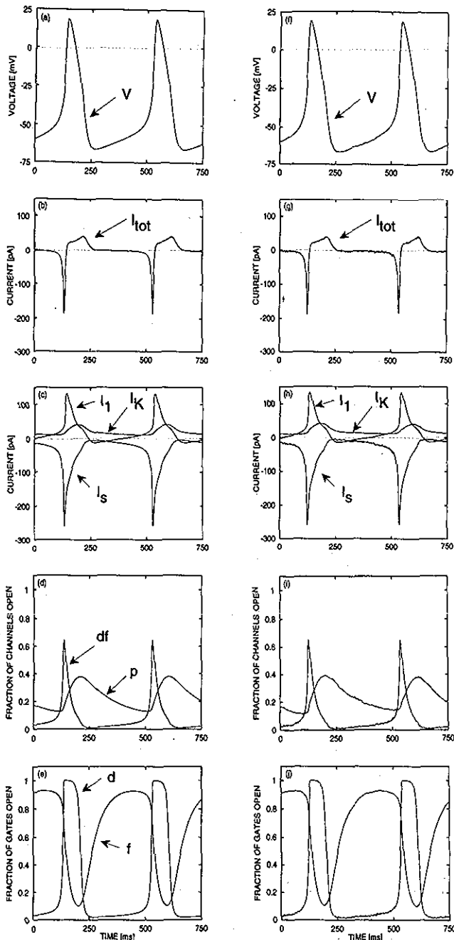
FIG. 3. 750 ms run of spontaneous activity in continuous (left panel) and single-channel (right panel) models. (a),(f) V ; (b),(g) I_{tot} ; (c),(h) I_s , I_K , I_L ; (d) df , p ; (i) fractions of I_s , I_K channels open; (e) d , f ; (j) fractions of d , f gates open. Initial conditions (left panel): V = -60 mV, d = 0.003 115 67, f = 0.910 749, p = 0.171 578. Initial conditions (right panel): V = -60 mV, fractions of gates open correspond to initial conditions on d , f , p as stated for the left panel. Not all data points computed are plotted. The "complex" simulation method was used in the right panel.
