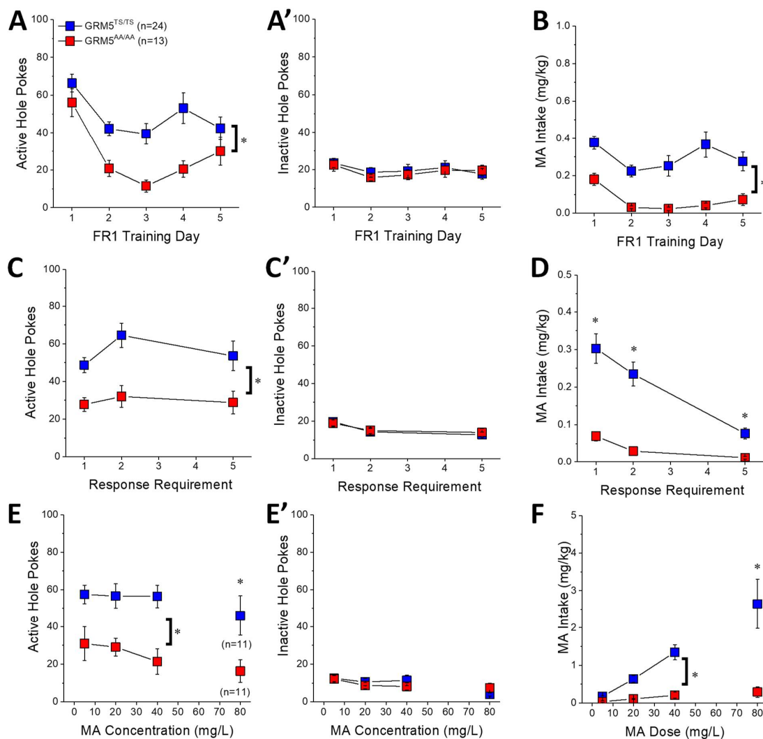
Figure 4. Disruption of ERK-dependent phosphorylation of mGlu5 blunts methamphetamine reinforcement and intake under operant-conditioning procedures. (Inset) Procedural timeline of the operant-conditioning studies conducted in Grm5 AA/AA and Grm5 TS/TS mice. When the first five days of self-administration training were considered, Grm5 AA/AA mutants exhibited less (A) methamphetamine (MA)-directed responding for reinforcement by 20 mg/L MA and (B) less MA intake than WT Grm5 TS/TS mice. When the response requirement for reinforcement by 20 mg/L MA progressively increased, mutant mice continued to exhibit (C) less MA-directed responding and (D) less intake. When the dose of the MA reinforcer varied under an FR1 schedule of reinforcement, the MA-directed responding (E) and MA intake (F) continued to be lower in Grm5 AA/AA mice versus Grm5 TS/TS controls. No genotypic differences were detected for responding in the inactive hole during (A') early training, (C') demand testing, or (E') dose-response testing. The data represent the means \pm SEMs of the number of mice indicated in parentheses. Note: not all mice tested for reinforcement by 5–40 mg/L MA advanced to testing under the 80 mg/L dose. * p < 0.05 (main Genotype effect); * p < 0.05 vs. Grm5 TS/TS ( t -test).
