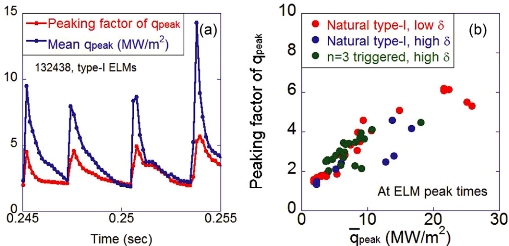
Figure 28. (a) Evolution of measured mean peak heat flux and toroidal peaking factor during type-I ELMs. (b) Toroidal peaking factor of q_{\text{peak}} during ELM activity occurring naturally, or triggered by 3D applied field pulses.
