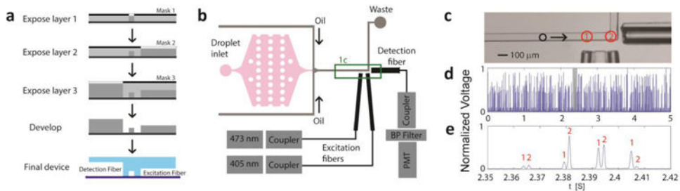
Figure 1. (a) Three layer lithographic fabrication of the device. Three layers of SU-8 are spun on and exposed to unique masks to give a combinations of 80 μm, 120 μm, and 220 μm tall geometries for flow channels and optical fibre inserts. (b) Layout of the device, including a schematic of the fibre coupled lasers and detector. The single detector, fibre-based approach requires a bandpass filter to exclude scattered laser light, a PMT, and three optical fibres. (c) Image of the detection region of the device, where the 473 nm laser excites region “1” and the 405 nm laser excites region “2” (d) Time series for 5 seconds of acquisition (e) Time series data from a train of 4 droplets containing different dye combinations
