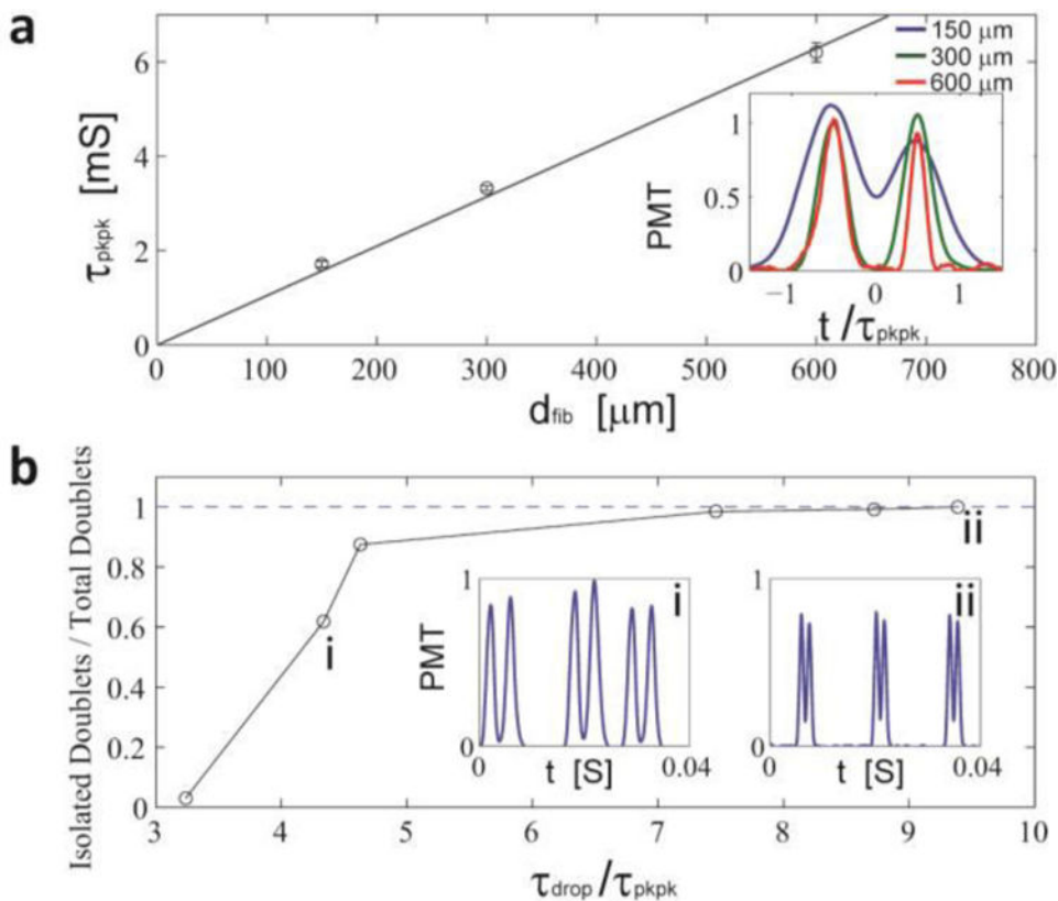
Figure 2. (a) Measured peak-peak delay time ( \tau_{pkpk} ) as a function of centre-to-centre fibre separation ( d_{fib} ). Inset gives normalized droplet signal shapes for different fibre-fibre separations. (b) The fraction of doublets from the total signal population isolated on each side by a region 2\tau_{pkpk} wide as a function of the normalized average droplet spacing. The insets show signal spacing data from the experiments at points marked i and ii.
