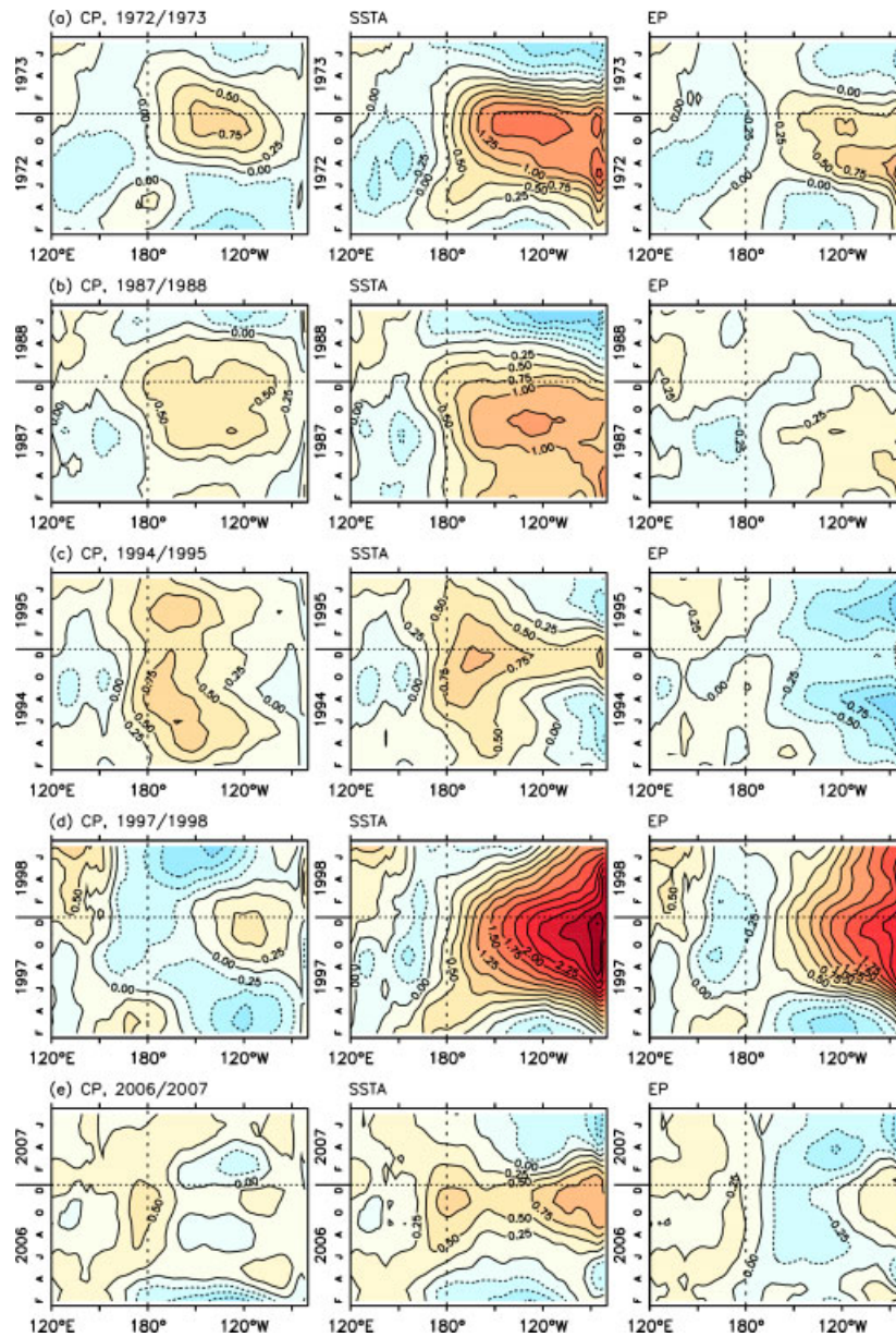
Figure 1. Longitude-time evolution of residual sea surface temperature (SST) anomalies for the CP type (left panels), total SST anomalies (middle panels), and residual anomalies for the EP type (right panels) averaged between 10°N and 10°S for (a) 1972/1973, (b) 1987/1988, (c) 1994/1995, (d) 1997/1998, and (e) 2006/2007 El Niño events.
