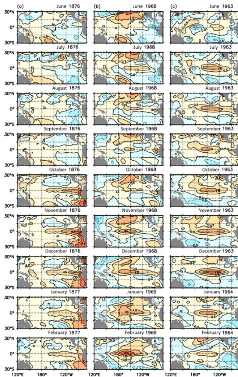
Figure 4. The spatial evolution of tropical SST anomalies from June of the El Niño year to February of the following year for (a) the 1876–1877 and (b) 1968–1969, (c) 1963–1964, (d) 1987–1988, and (e) 2006–2007 events.
