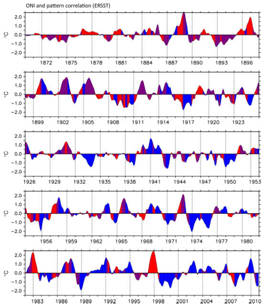
Figure 3. Time series of the ONI with pattern correlation difference superimposed. The red colour indicates EP type, blue colour CP type, and blended colour mixed type.
