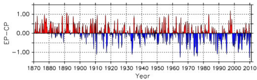
Figure 2. Time series of pattern correlation difference (EP-CP). The pattern correlations are estimated for the regions 120^{\circ}\text{E}-70^{\circ}\text{W} and 10^{\circ}\text{N}-10^{\circ}\text{S} .
