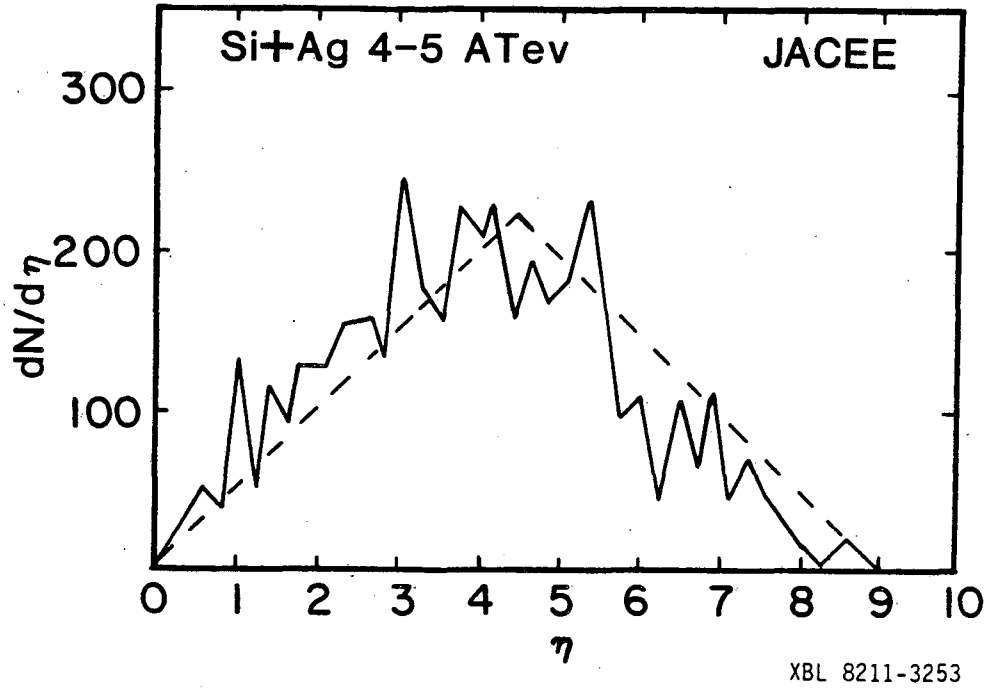
Fig. 5 Pseudo rapidity distribution 12) of Si (4-5 ATeV) + Ag \gg 1000 charges + X. The most spectacular nuclear collision ever recorded! Dashed triangle is to guide the eye.
