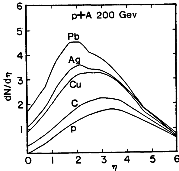
Fig. 4 Pseudo rapidity ( \eta = -\ln \tan \theta_{\text{Lab}}/2 ) distributions of particles produced in p + A collisions at 200 GeV. 5
