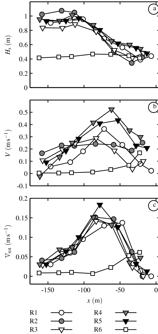
Figure 2.2: (a) Significant wave height H_s , (b) mean alongshore current V , and (c) horizontal rotational velocities V_{\text{rot}} versus cross-shore distance from the shoreline x for each dye release (see legend).
