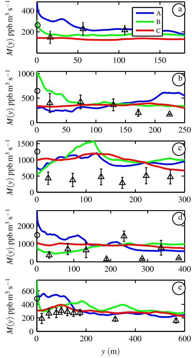
Figure 4.5: Modeled M^{(A,B,C)} (colored curved) and observed M^{(\text{obs})} transect estimated (black triangles with error bars) alongshore tracer fluxes (4.2) vs y , for releases (a) R1, (b) R2, (c) R3, (d) R4, and (e) R6. The observed pumped dye release rate is estimated by the black circle at y = 0
