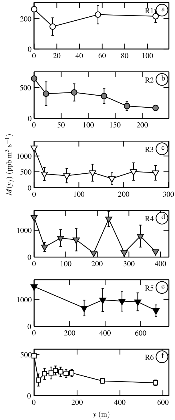
Figure 2.9: Tracer alongshore transport M(y_j) (2.5) versus y , with error bars \pm \epsilon_M for releases (a) R1, (b) R2, (c) R3, (d) R4, (e) R5, and (f) R6. The initial condition at y = 0 m is the injected dye transport (concentration times flow-rate).
