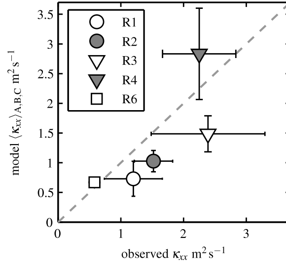
Figure 4.8: Mean modeled \langle \kappa_{xx} \rangle_{A,B,C} vs observed \kappa_{xx}^{(\text{obs})} , with a dashed line indicating perfect agreement. The \kappa_{xx}^{(\text{obs})} error bars are estimated from the \sigma_{\text{surf}}^{2(\text{obs})} versus t_p fit slope error [Clark et al. , 2010], and model \langle \kappa_{xx} \rangle_{A,B,C} error bars are the combination of fit slope errors and the variation in \kappa_{xx}^{(A,B,C)} magnitudes. The skill (relative to perfect agreement) is 0.40.
