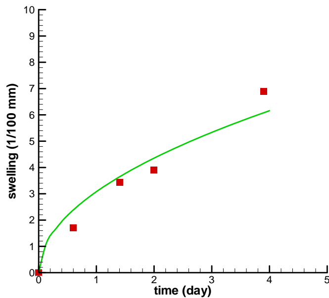
Figure 3. Match between observed swellings for points (3, 4, 7, 10, and 14) with those calculated from Eq (8) (solid curve).
