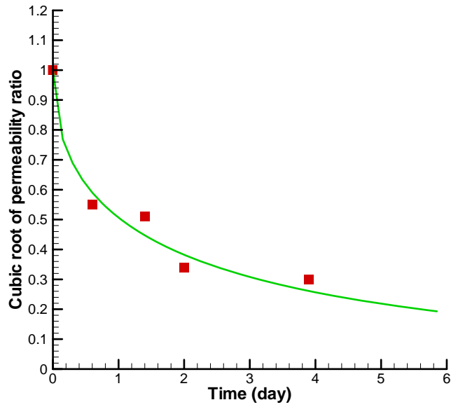
Figure 4. Match between observed values for (k/k_3)^{1/3} for points (3, 4, 7, 10 and 14) with those calculated from Eq. (11) (solid curve). The fitted B value is 0.68 \text{ d}^{-1/2} .
