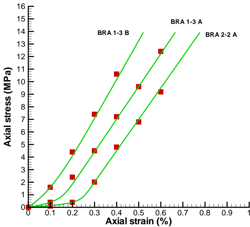
Figure 1. Matches between laboratory measurements and Eq (8) in which volumetric strain and a bulk modulus ( K ) need to be replaced with axial strain and the corresponding Young's modulus ( E ), respectively. The data points are measurements (Corkum and Martin, 2007) and the solid curves are theoretical results.
