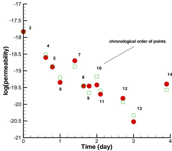
Figure 5. Comparisons between observed and simulated fracture permeability changes as a function of time. The solid circles are measurements.
