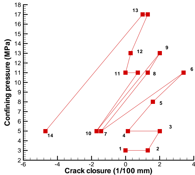
Figure 2. Test procedure of water permeability measurement (in terms of confining pressure and fracture [crack] closure) for sample 2 of Davy et al. (2007). The numbers in the figure indicate the chronological order of points (Catherine A. Davy, Personal communication). Since measured crack closure in Davy et al. (2007) is actually an effective parameter representing displacement of bulk rock sample, it can be positive or negative depending on the combination of confining pressure and swelling
