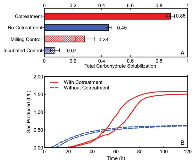
Fig. 3 (A) Final solubilization of senescent switchgrass and (B) gas production throughout fermentation by C. thermocellum with and without cotreatment. Solubilization bar plots are at least n = 3 with error bars representing one standard deviation.
