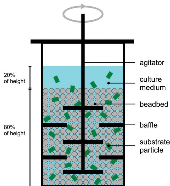
Fig. 1 Schematic of the cotreatment reactor with baffles and bed height shown.
