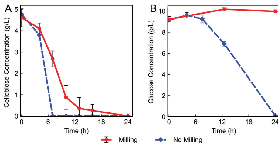
Fig. 2 (A) Cellobiose consumption by C. thermocellum and (B) glucose consumption by S. cerevisiae D 5 A with and without ball milling (duplicate fermentations with error bars representing one standard deviation).
