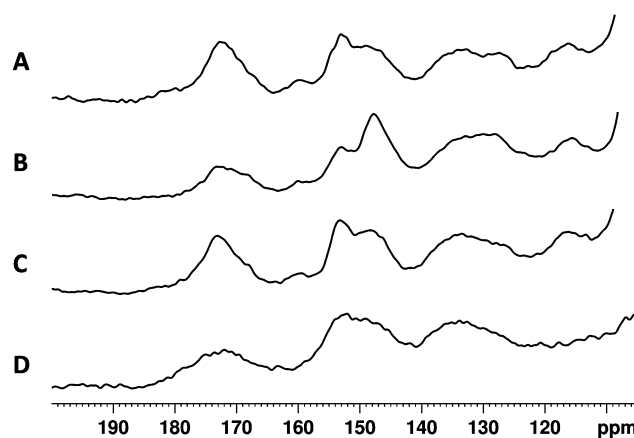
Fig. 6 Aromatic region of solid-state 13 C cross polarization magic angle spinning (CP/MAS) spectra of switchgrass feedstock before and after conversion. (A) Switchgrass feedstock before conversion. (B) Residue after hydrothermal pretreatment. (C) Residue remaining after C. thermocellum fermentation. (D) Residue remaining after C. thermocellum cotreatment following removal of metal particles by sonication after suspension in an EDTA solution.
