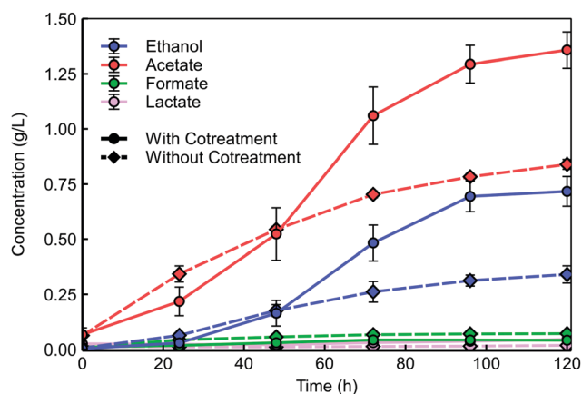
Fig. 4 Major fermentation products by C. thermocellum when grown on senescent switchgrass with and without cotreatment, data are at least n = 4 and error bars represent 1 standard deviation.
