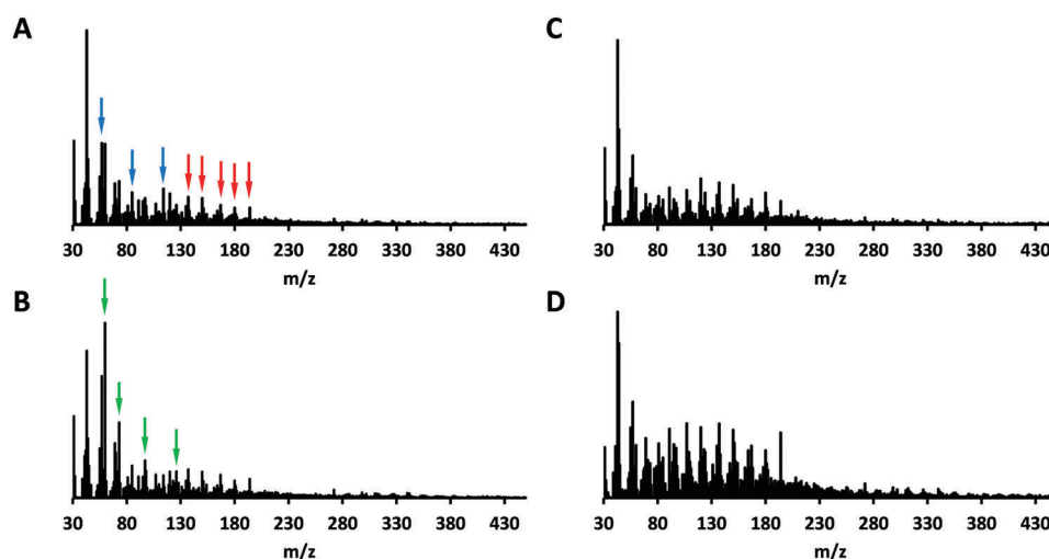
Fig. 5 PyMBMS spectra of switchgrass feedstock before and after conversion. (A) Switchgrass feedstock before conversion. Blue arrows highlight monomers released during pyrolysis derived from xylan. Red arrows highlight monomers released during pyrolysis derived from lignin. (B) Residue after hydrothermal pretreatment. Green arrows highlight monomers released during pyrolysis derived from C6 sugars, predominately cellulose. (C) Residue remaining after C. thermocellum fermentation without cotreatment. (D) Residue remaining after C. thermocellum fermentation with cotreatment.
