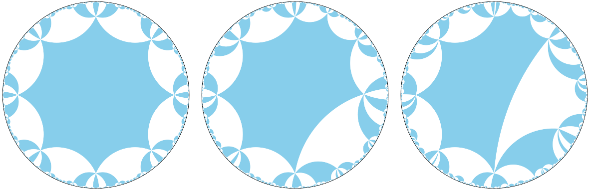
Figure 2.2: The evolution of the Fenchel–Nielsen twist flow on the hyperbolic surface of Example 2.2.1.
