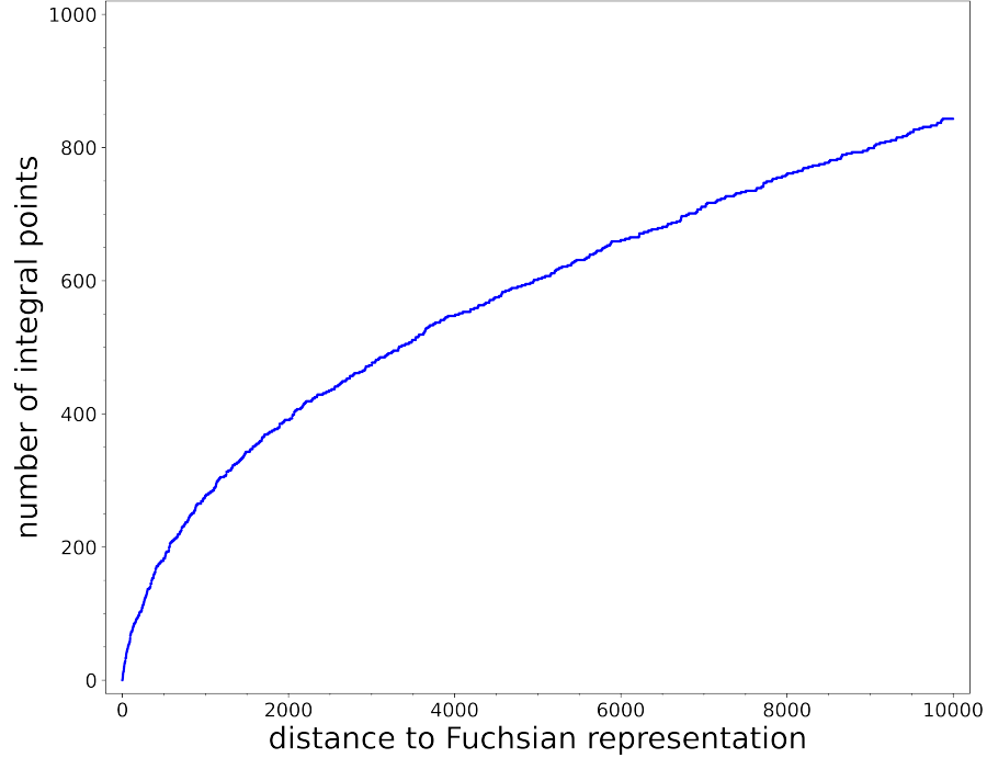
Figure 4.3: Distributions of representations in \mathcal{H}_3(X_{3,3,4})_{\mathbf{Z}} .
