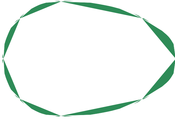
(c) Bulging as a convex projective structure.
