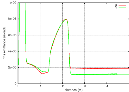
Figure 2. Transverse emittance evolution at LCLS photoinjector with initial 0.5 mm offset from IMPACT-T simulation.
