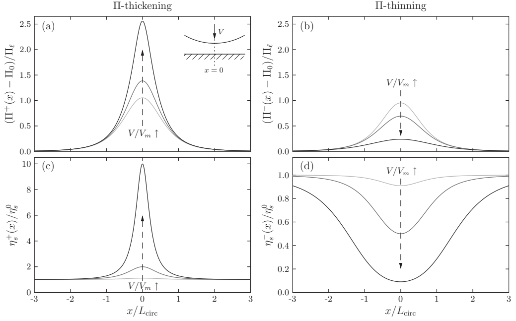
FIG. 4. Pressure and viscosity distributions in the gap between an approaching disk and a wall for a \Pi -thickening (a, c) and a \Pi -thinning surfactant (b, d). In the \Pi -thickening case, the approach velocity can not exceed a maximum value V = V_m , with V/V_m = 0.1, 0.5 , and 0.9 depicted. No maximum approach velocity exists for \Pi -thinning surfactants. Lines correspond to V/V_m = 0.1, 1 , and 10 .
