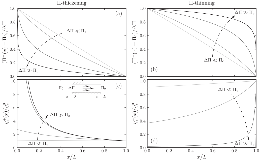
FIG. 3. Pressure and viscosity distributions in a channel for a \Pi -thickening (a, c) and a \Pi -thinning surfactant (b, d). The lines correspond to \Delta\Pi/\Pi_c = 0.1, 1, 4 , and 10 , with the dashed arrow indicating the direction of increasing \Delta\Pi in each case.
