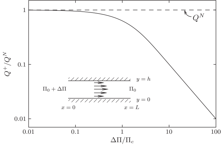
FIG. 2. Flux Q^+ of a \Pi -thickening surfactant driven through a channel, compared with its Newtonian analog ( Q^N ). While Q^N increases linearly with the applied pressure difference \Delta\Pi , Q^+ approaches a constant when \Delta\Pi \gtrsim \Pi_c .
