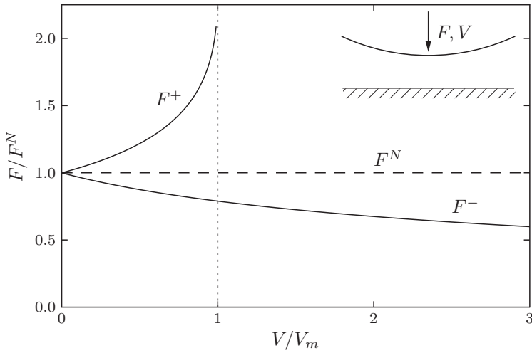
FIG. 5. Force-velocity relations for a circular disk approaching a wall in \Pi -thickening and \Pi -thinning mediums. The vertical dotted line represents the maximum velocity of approach in a \Pi -thickening surfactant, at which point the force diverges.
