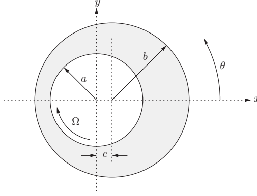
FIG. 6. Geometry of the journal bearing.
