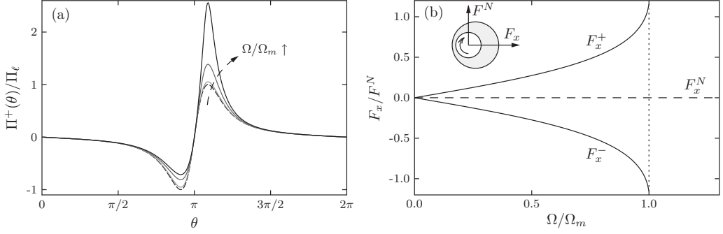
FIG. 7. (a) Pressure distribution in a \Pi -thickening surfactant in a 2D journal bearing. For the sake of illustration, we choose \lambda = c/(b - a) = 0.9 in this case. The arrow points to the direction of increasing angular velocity, with \Omega/\Omega_m = 0.1, 0.5 , and 0.9 . The dashed line is the Newtonian pressure distribution \Pi^N(\theta) . (b) Radial (or horizontal, in the geometry of Fig. 6) force on the inner cylinder. For a Newtonian fluid, F^N = F_y^N and F_x^N = 0 .
