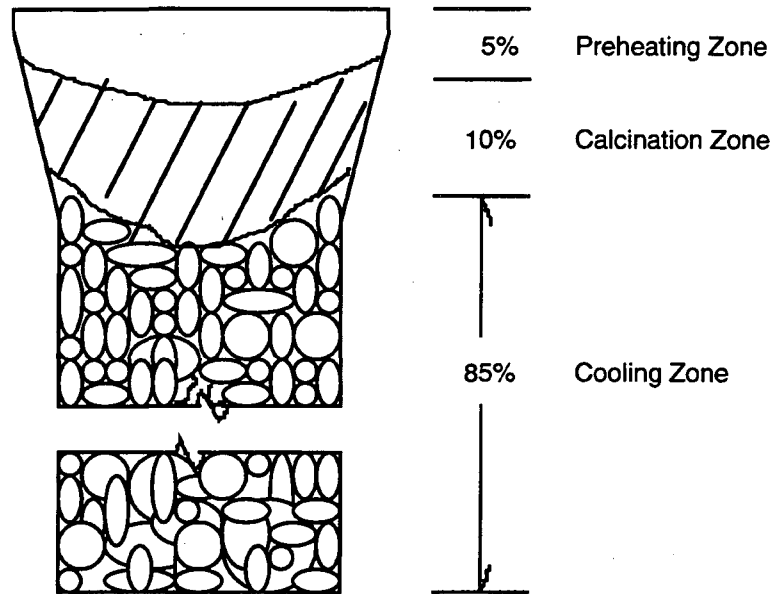
Figure 3-2. The Basic Structure of Vertical Kilns
