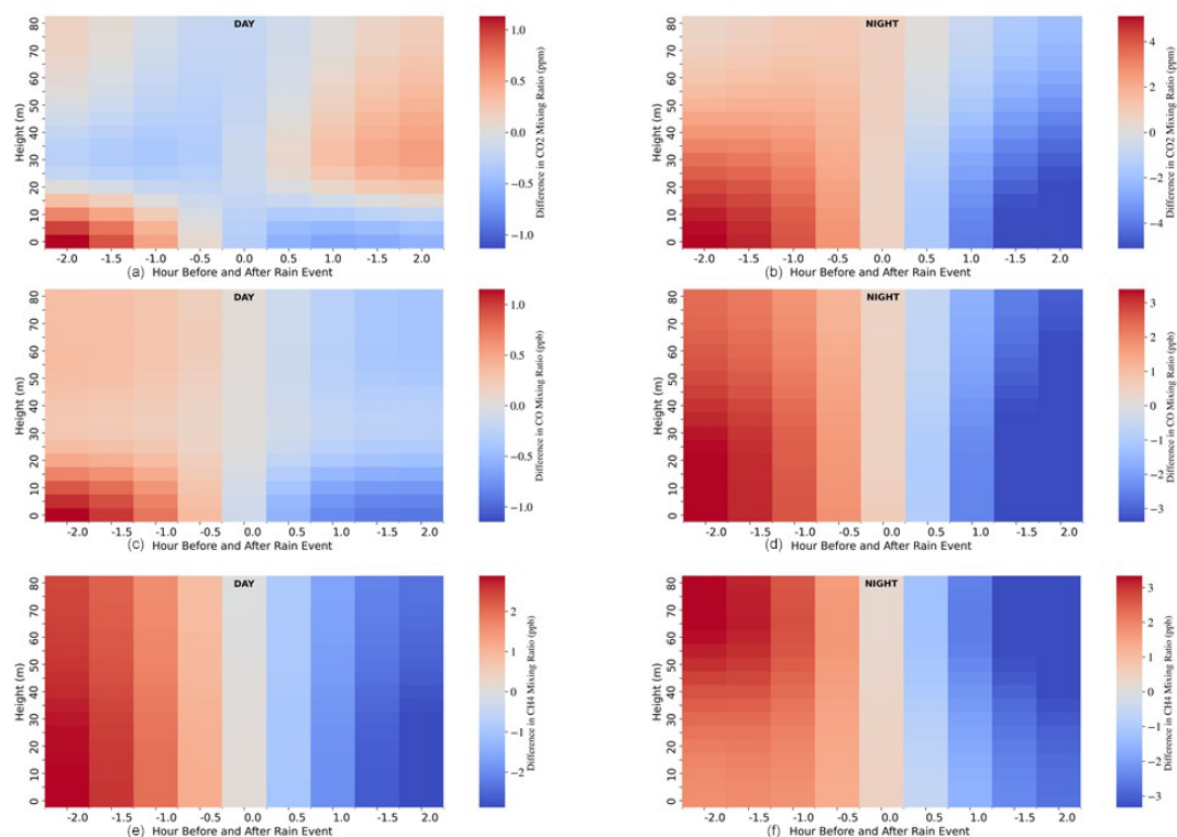
Figure 4. Composite of CO 2 during the day (a) and night (b), CO during the day (c) and night (d), and CH 4 during the day (e) and night (f) for 2 h before the maximum rain rate to 2 h after. Please note that the color bar scale is different between each figure. A rainfall event was considered to be an event with at least one case with a rain rate larger than 0.5 mm h -1 . Calculation was done for all cases from January 2013 to December 2020. Values are presented as the deviation from median composite values.
