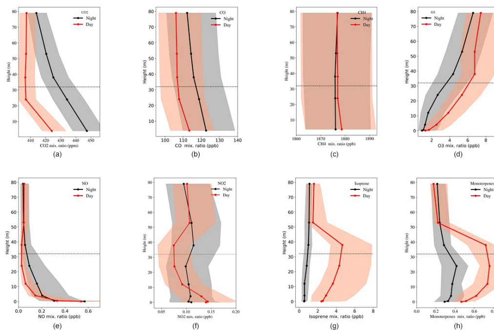
Figure 1. Vertical profiles of median mixing ratios and 30th and 70th percentile intervals (shading) for (a) \text{CO}_2 , (b) \text{CO} , (c) \text{CH}_4 , (d) \text{O}_3 , (e) \text{NO} , (f) \text{NO}_2 , (g) isoprene, and (h) monoterpenes during the day (red) and night (black) for all rain events. The dataset to compute the median spans a 2 h window before and after the peak rain rate. The total number of rain events for each gas is detailed in the “Data analysis” section.
